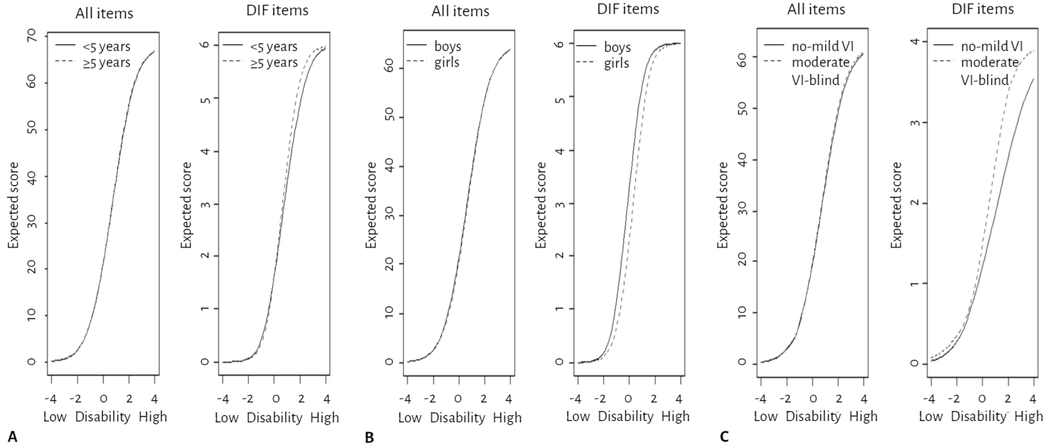
Figure 1. Total impact of DIF on the test characteristic curve (TCC) for age (A), gender (B), and level of VI (C)
