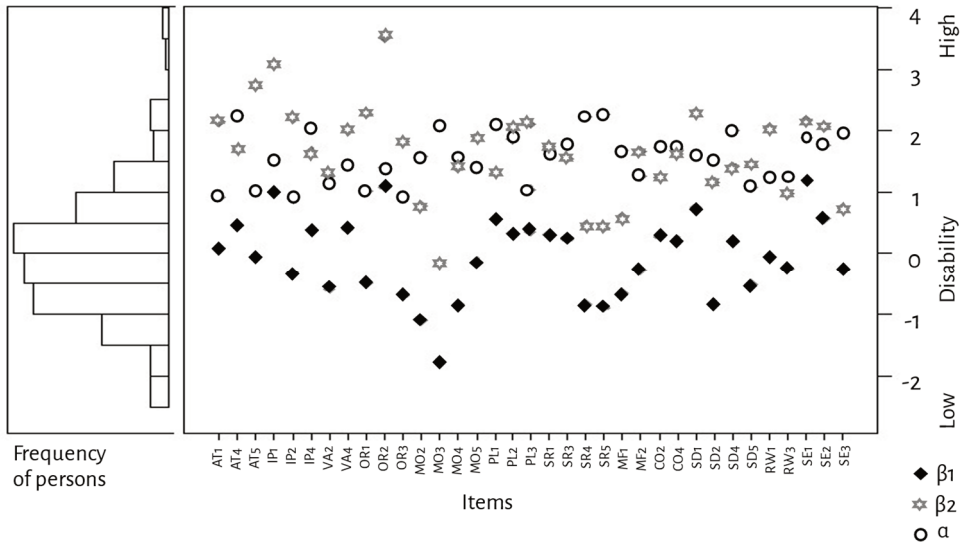
Figure 2. Item-person map of the 35-item PAI-CY 3-6
