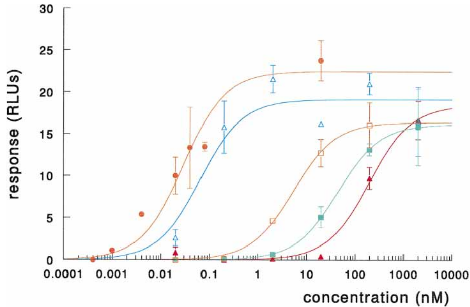
Fig. 2. Response of 17 \beta -estradiol (closed circles), 4-hydroxy-17 \beta -estradiol (open triangles) 4-hydroxy-17 \beta -estrone (open squares), 2-hydroxy-17 \beta -estrone (filled squares), and 2-hydroxy-17 \beta -estradiol (filled triangles) in the ER-CALUX assay. Results are expressed as the mean \pm SEM (n=3). The response obtained with the solvent control is subtracted. Data were fitted by 1-ligand curve fitting.
