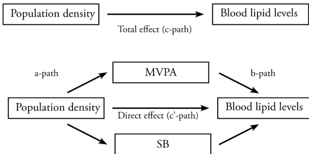
Figure 2 Mediation analysis framework.
