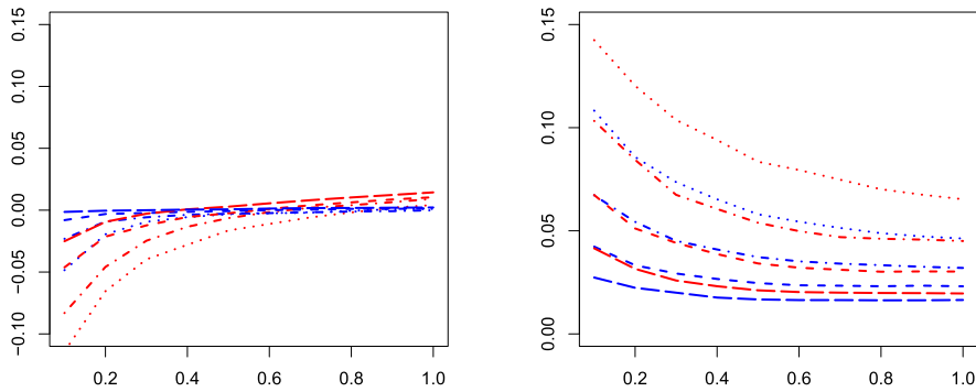
Figure 4. For the bandwidth b varying in [0.1, 1] calculation of the empirical bias (left plot) and standard deviation (right plot) of N = 1000 estimates of \theta_0 = 0.5 for an ARA_1 model (red) and an ARA_\infty model (blue) with sample size n = 50 (dotted lines), n = 100 (dashed dotted lines), n = 200 (dashed lines), n = 500 (long dashed lines) for Type-II censoring with k = 4 ( s sufficiently large).
