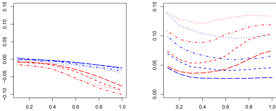
Figure 3. For the bandwidth b varying in [0.1, 1] calculation of the empirical bias (left plot) and standard deviation (right plot) of N = 1000 estimates of \theta_0 = 0.5 for an \text{ARA}_1 model (red) and an \text{ARA}_\infty model (blue) with sample size n = 50 (dotted lines), n = 100 (dashed dotted lines), n = 200 (dashed lines), n = 500 (long dashed lines) for Type-I censoring with \tau = s = 5 .
