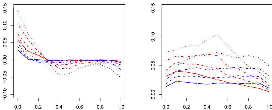
Figure 2. Empirical bias (left plot) and standard deviation (right plot) based on N = 1000 estimates of \theta_0 varying in [0, 1] for an ARA_1 model (red) and an ARA_\infty model (blue) with sample size n = 50 (dotted lines), n = 100 (dashed dotted lines), n = 200 (dashed lines), n = 50 (long dashed lines) for Type-II censoring with k = 4 ( s sufficiently large) and bandwidth b = 0.3 .
