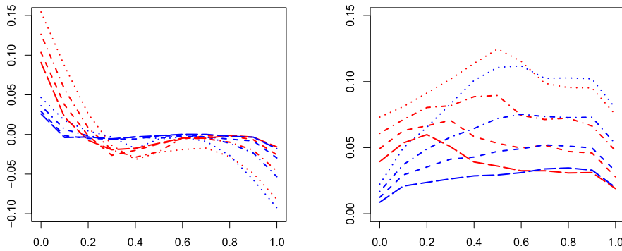
Figure 1. Empirical bias (left plot) and standard deviation (right plot) based on N = 1000 estimates of \theta_0 varying in [0, 1] for an ARA_1 model (red) and an ARA_\infty model (blue) with sample size n = 50 (dotted lines), n = 100 (dashed dotted lines), n = 200 (dashed lines), n = 400 (long dashed lines) for Type-I censoring with \tau = s = 5 and bandwidth b = 0.3 .
