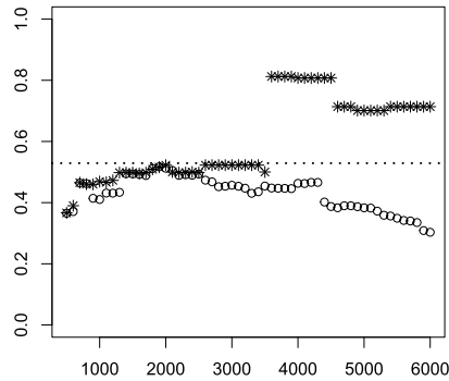
Figure 7. Maximizers of the smoothed profile likelihood function based on (2.4) (stars) or on (5) (circles).
