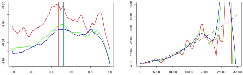
Figure 6. On the left-hand side are the profile likelihood functions for b = 1000 (red), b = 2000 (green) and b = 3000 (blue), the vertical lines correspond to the locations of the maxima whereas the black dashed vertical line corresponds to the parametric estimate in [10]. On the right-hand side are the corresponding estimates of the baseline hazard rate function, the black dashed curve corresponds to the parametric estimator in [10].
