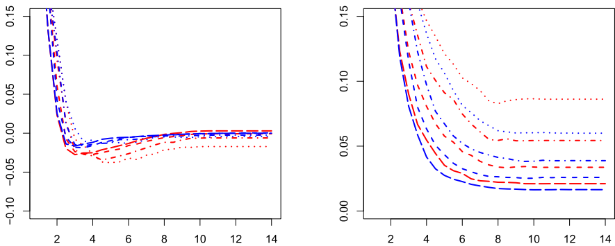
Figure 5. For s varying in [1, 14] calculation of the empirical bias (left plot) and standard deviation (right plot) of N = 1000 estimates of \theta_0 = 0.5 for an ARA_1 model (red) and an ARA_\infty model (blue) with sample size n = 50 (dotted lines), n = 100 (dashed dotted lines), n = 200 (dashed lines), n = 500 (long dashed lines) for Type-II censoring with k = 4 and bandwidth b = 0.5 .
