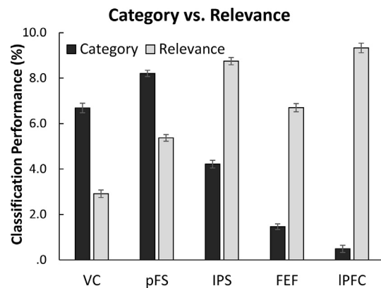
Fig. 3 – Delay interval: Direct comparison of category decoding versus relevance (status) decoding. Here classification performance is shown collapsed across the three sub conditions (current, prospective, irrelevant) and with chance level subtracted (33.33% for category decoding, 50% for relevance decoding). Error bars indicate Standard Error of the mean (SE).
