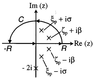
FIG. 9. Integration path in the complex plane used to evaluate Eq. (21). The same path can be used to evaluate Eq. (33), by replacing \xi_p \pm i\beta with \xi_p \pm i\sigma .
