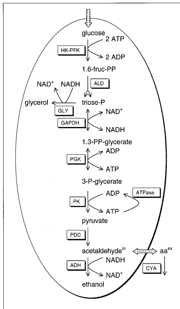
FIGURE 1 Schematic representation of the anaerobic glycolytic pathway. Reactions: HK-PFK, lumped reaction of hexokinase and phosphofruktokinase; ALD, aldolase reaction; GLY, glycerol-producing branch; GAPDH, reaction of glyceraldehyde-3-phosphate dehydrogenase; PGK, reaction catalyzed by phosphoglycerate kinase; PK, lumped reactions of phosphoglycerate mutase, enolase, and pyruvate kinase; PDC, reaction catalyzed by pyruvate decarboxylase; ADH, alcohol dehydrogenase reaction; ATPase, total cellular ATP consumption; CYA, degradation of acetaldehyde by cyanide. Fluxes: glucose influx, exchange of acetaldehyde between the cell and the external medium.
