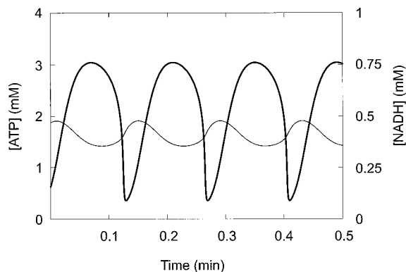
FIGURE 4 Integration of NADH and ATP of the 9-variable model in time. The period of the oscillation is T = 0.141 min, phaseshift of NADH ( thin line ) and ATP ( thick line ) equals 152^\circ . Parameters as in Table 1, and k_0 = 80.0 \text{ min}^{-1} .
