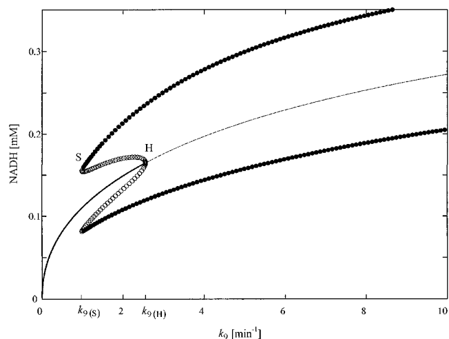
FIGURE 3 Bifurcation diagram for the variable N_2 (NADH) in mM. The bifurcation parameter k_0 is the pseudo-first-order rate constant of the extracellular degradation of acetaldehyde. Solid line , stable steady state; dashed line , unstable steady state. Empty circles , maxima and minima of unstable limit cycles; full circles , maxima and minima of stable limit cycles. Points: S, point of a saddle-node bifurcation of the limit cycle; H, point of Hopf bifurcation. Parameters as given in Table 1.
