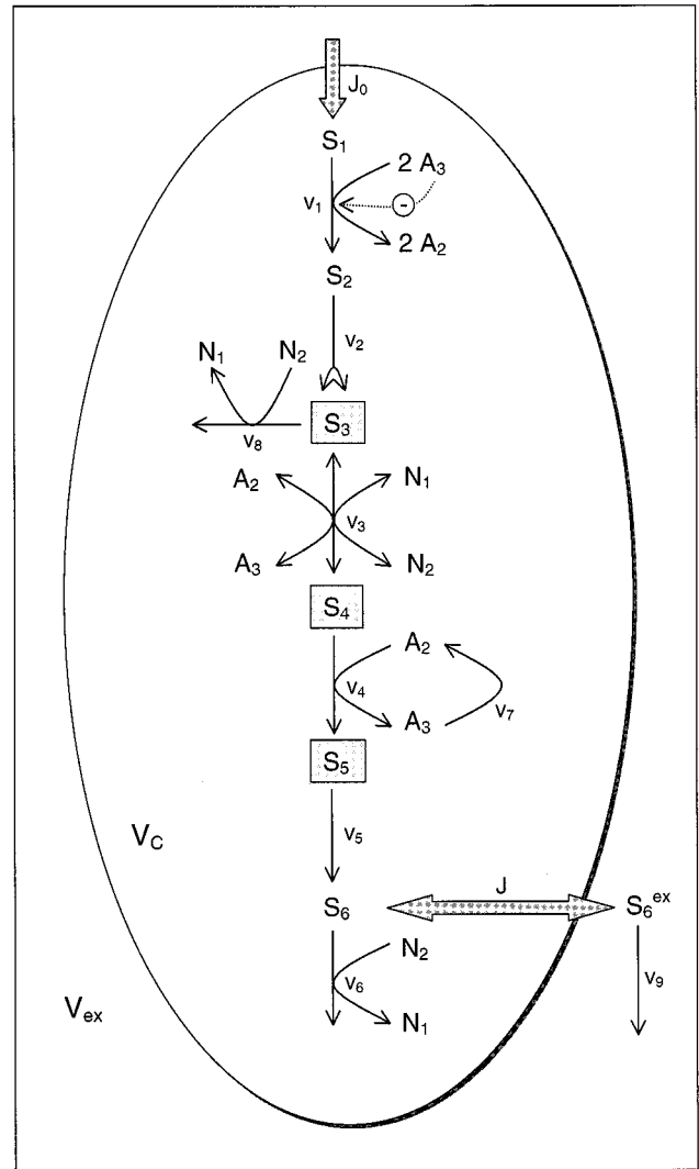
FIGURE 2 Schematic representation of the models. The 9-variable model includes all shown metabolites as variables, whereas, in the 6-variable model S_3 , S_4 , and S_5 are treated as parameters. Variables: S_1 , glucose; S_2 , fructose-1,6-bisphosphate; S_3 , pool of the triosephosphates, glyceraldehyde-3-phosphate, and dihydroxyacetone phosphate; S_4 , 3-phosphoglycerate; S_5 , pyruvate; S_6 , acetaldehyde in the cell; S_6^{ex} , extracellular acetaldehyde; A_3 , ATP, and N_2 , NADH.
