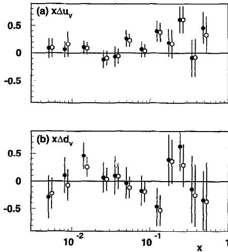
Fig. 4. Quark spin distribution functions (a) x\Delta u_v(x) and (b) x\Delta d_v(x) obtained from the asymmetries A^{+-} (Eq. (6), open circles) and the asymmetries A^{+} and A^{-} (Eq. (2), closed circles) without using inclusive asymmetries and without the constraint \Delta\bar{u} = \Delta\bar{d} . Errors are statistical.
