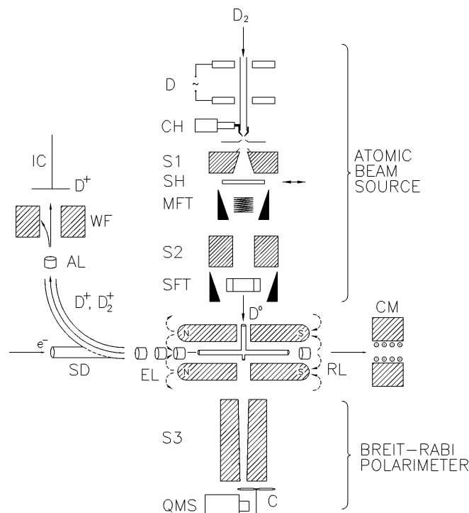
FIG. 1. Schematic outline of the atomic beam source, Breit-Rabi polarimeter, internal target, and ion-extraction system. All components, except the target holding field and correction magnets, are inside the vacuum system. D: rf dissociator; CH: cold head; S1, S2, S3: sextupole magnets; MFT, SFT: medium- and strong-field transition units; SH: shutter; C: chopper; QMS: quadrupole mass spectrometer; CM: correction magnet; RL: repeller lens; EL: triplet of ion-extraction lenses; SD: spherical deflector; AL: electrostatic lens; WF: Wien filter; IC: ion collector.
