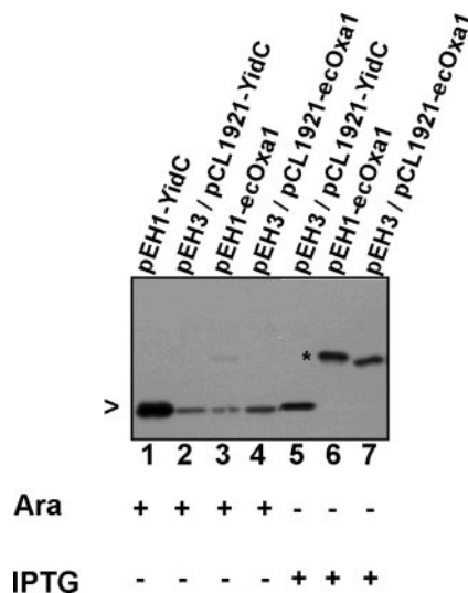
FIG. 3. Expression of YidC and ecOxa1 in the YidC depletion strain JS7131. Strain JS7131 harboring the indicated constructs was grown in LB medium in the presence of 0.2% L-arabinose (lane 1–4) or IPTG (50 \mu M, lane 5–6; 1 mM, lane 7). Cell samples were taken at mid-log phase, and 0.05 OD 660 units of cells were analyzed by SDS-PAGE and immunoblotting for YidC and ecOxa1 content using YidC antiserum. The position of ecOxa1 is indicated by an asterisk, and the position of YidC is indicated by an arrowhead.
