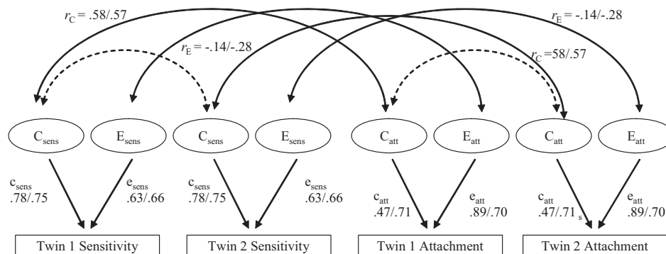
Figure 2. Parameter estimates for the structural equation model of sensitivity and attachment. The path coefficients are standardized and represent the effect with (before the '/') and without (after the '/') Disorganized cases included in the analysis. C and E refer to shared environmental and nonshared environmental latent variables, respectively. Lowercase c and e refer to the effects (path coefficients) of these respective latent variables on the measured variables. Shared and nonshared environmental latent variables and path coefficients for sensitivity and attachment are distinguished by the subscripts sens and att , respectively.
