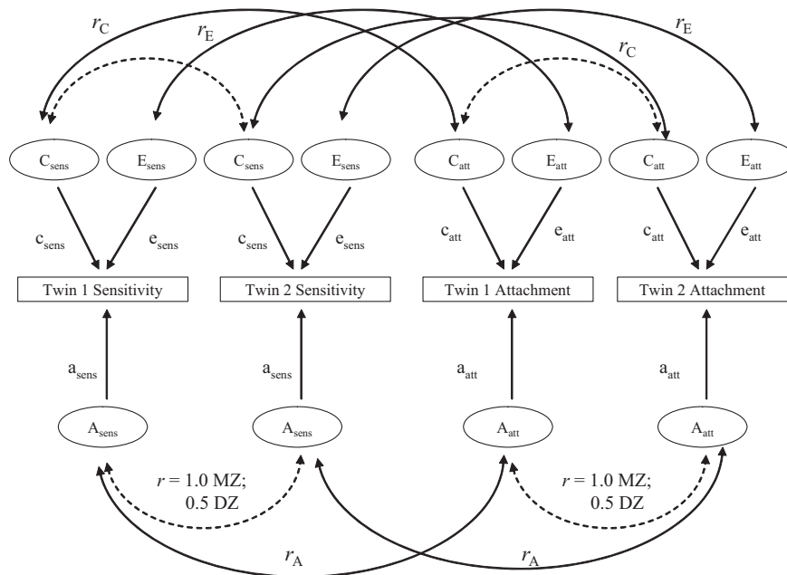
Figure 1. Path diagram of the bivariate genetic model. A, C and E refer to genetic, shared environmental and nonshared environmental latent variables, respectively. Lowercase a, c and e refer to the effects (path coefficients) of these respective latent variables on the measured variables. Genetic and environmental latent variables and path coefficients for sensitivity and attachment are distinguished by the subscripts sens and att , respectively. MZ = monozygotic twins; DZ = dizygotic twins.
