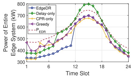
Fig. 9. Comparison of the entire edge system power within the edge demand response event with different mechanisms.
