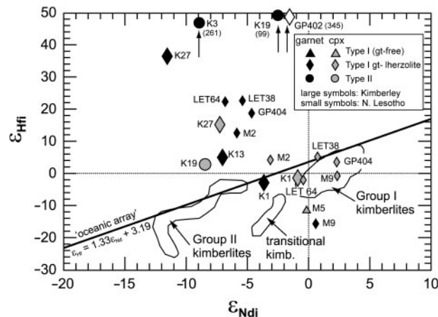
Fig. 10. \epsilon_{Hf1} vs \epsilon_{Nd1} isotope diagram showing the data for garnets and cpx from xenoliths from Lesotho and Kimberley. The fields for Group I, Group II and transitional kimberlites are also shown (data from Nowell et al. , 2004). Oceanic mantle array (regression line through ocean island and mid-ocean ridge basalt data) from Vervoort & Blichert-Toft (1999). K27, K19 and K3 garnets plot outside the diagram in \epsilon_{Hf1} (values in parentheses, Table 4).
