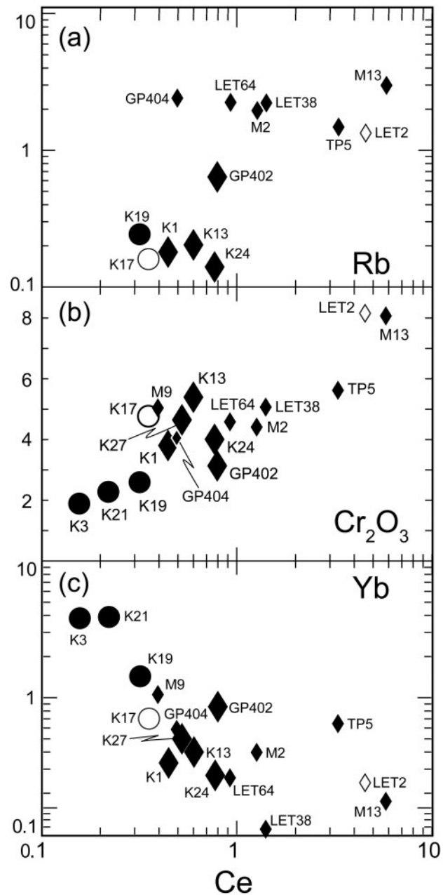
Fig. 15. Correlation of LREE (Ce) content in garnet with (a) \text{Rb} , (b) \text{Cr}_2\text{O}_3 (wt%) and (c) \text{Yb} . All but \text{Cr}_2\text{O}_3 in ppm. Symbols are as in Fig. 6.
