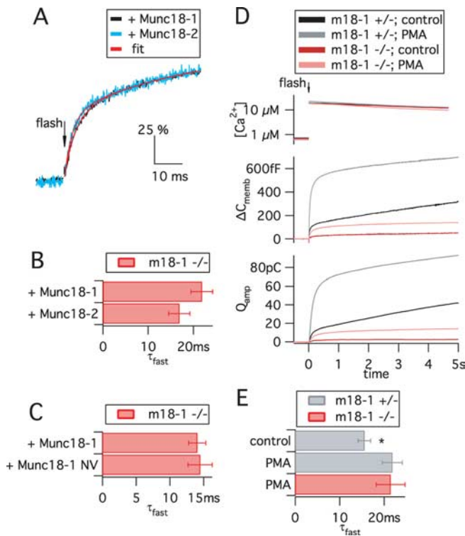
Figure 7. The absence or presence of Munc18 variants does not affect fusion triggering. A–C , Kinetics of the fusion of primed vesicles, triggered by \text{Ca}^{2+} uncaging and assayed by membrane capacitance recordings. Data are from recordings presented in Figures 5 and 6 and supplemental Table 1 (available at www.jneurosci.org as supplemental material). A , The time courses of responses in the presence of Munc18-1 and Munc18-2 (normalized to the burst amplitude, 100%) are similar despite the large difference in the absolute \Delta C_{\text{memb}} amplitude (refer to Fig. 5A). A double-exponential function (red lines) was fitted to data points (black and blue traces). B , C , The faster time constant of the exponential fits ( \tau_{\text{fast}} ; mean \pm SEM) was statistically indistinguishable between Munc18-1, Munc18-2, and Munc18-1 NV. For other parameters, refer to supplemental Table 1 (available at www.jneurosci.org as supplemental material). D , PMA treatment increased exocytosis in both munc18-1 -/- and munc18-1 +/- cells by approximately the same factor, showing that the PMA potentiation in embryonic mouse chromaffin cells is not dependent on Munc18-1. Data are means of n = 28 +/- control cells, 31 +/- PMA cells, and 32 -/- PMA cells. E , After PMA treatment, kinetic analysis was possible in munc18-1 -/- cells. Shown is the \tau_{\text{fast}} from +/- and -/- cells. PMA treatment mildly increased the \tau_{\text{fast}} of +/- cells (* p < 0.05 ), but deletion of Munc18-1 had no effect in the presence of PMA.
