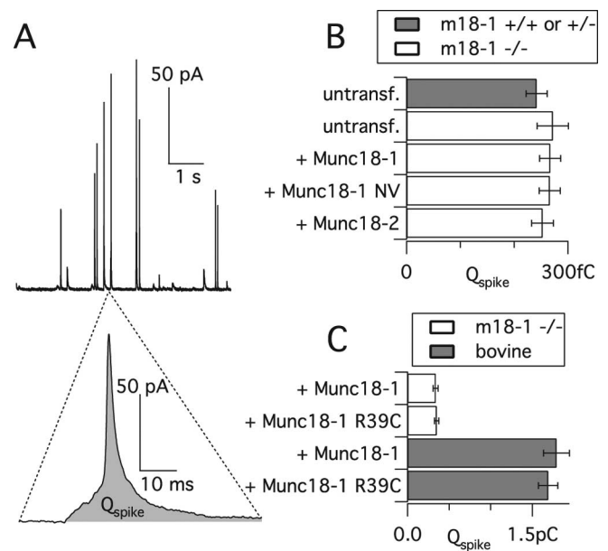
Figure 8. Single fusion events are unchanged by mutation or deletion of Munc18-1. Kinetics of single fusion events, assayed by carbon fiber amperometry, during sustained stimulation by extracellular \text{K}^{+} . A , Amperometric spikes (top) from a munc18-1 -/- cell expressing Munc18-1. Note the prespike foot in the expanded trace (bottom). B , Total charge ( Q ) of the spikes recorded from munc18-1 -/- , +/-, or +/- cells, or -/- cells expressing different Munc18 constructs. Shown is the mean of cell medians. For statistics of other parameters, see Table 1. C , Comparison of Munc18-1 R39C with Munc18-1 expressed in either munc18-1 -/- mouse cells or bovine cells.
