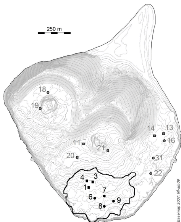
Figure 1. Location of the permanent study plots on Surtsey that were sampled in the study, shown on a topographical map from 2007. Contour intervals are 2 m, the highest point of the island is 152 m a.s.l. The sea bird colony plots in the southern part are marked with the solid line and black plot numbers. Outside the colony the plots have grey plot numbers. Circles indicate plots with shallow soils (< 10 cm soil depth), squares indicate plots with deep soil ( \geq 30 cm soil depth).
