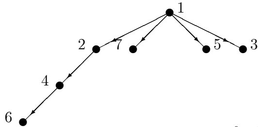
Figure 3: Hierarchy (N^6, S^6)
