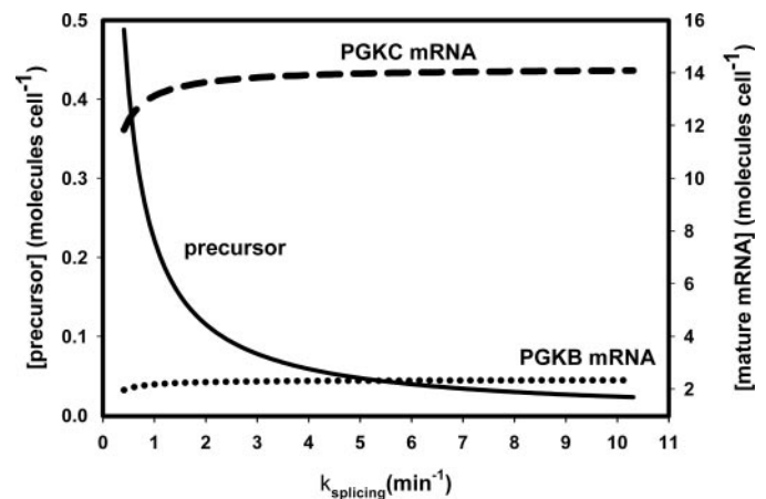
FIGURE 4. Modeled relationship between k_{\text{splicing}} and precursor and mRNA concentrations.
