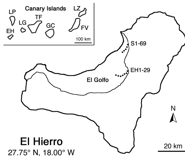
Figure 1. El Hierro and the Canary Islands. El Hierro (EH) is the most westerly of the Canaries. The other islands are (from west to east) La Palma (LP), La Gomera (LG), Tenerife (TF), Gran Canaria (GC), Fuerteventura (FV) and Lanzarote (LZ). The dashed lines indicate our section, Camino de Jinama (EH1-29), and Széréméta et al. (1999)'s section a few kilometres to the north (S1-69) along the El Golfo scarp.
