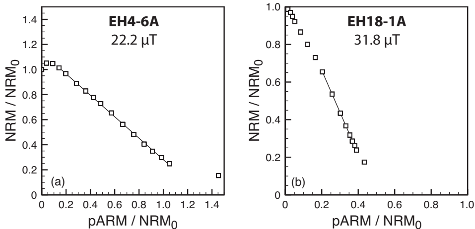
Figure 7. Calibrated pseudo-Thellier results. The pseudo-Thellier slopes are generally very linear, as illustrated by the results of samples EH4-6A (a), and EH18-1A (b). Minor non-linear behaviour is visible for the lower alternating field levels (top left points) and the highest alternating field levels (bottom right points). The most linear segment is interpreted.
