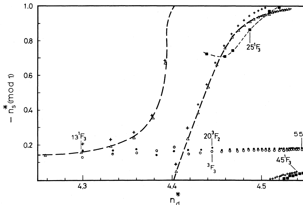
FIG. 2. Partial Lu-Fano plot of ^1F_3 states (+), ^3F_2 states (●), and ^3F_3 states (○). The position of ^1F_3 states predicted from Stark effect data (Ref. 11) (Δ) and hyperfine structure (Ref. 5) (■) are included. The curves through the various sets of data points serve to guide the eye.
