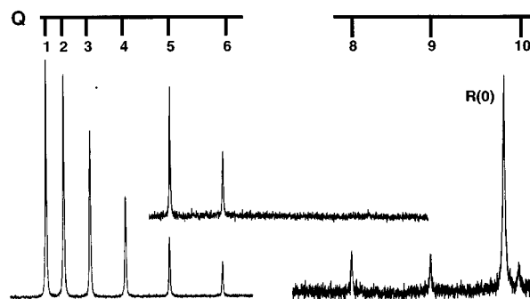
Fig. 4. Excitation spectrum of the L^1\Pi - X^1\Sigma^+(0,0) band of CO in the bandhead region of the Q branch by 1XUV + 1UV photoionization at \lambda = 96.83 nm, recorded in three separate overlapping scans. Note that the Q(7) line is missing.
