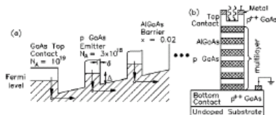
FIG. 1. (a) A partial band diagram of the top two periods for a HEIWIP detector using doped GaAs as the emitter layer and undoped AlGaAs as the barrier with the work function \Delta (the difference between the barrier energy and the fermi energy) indicated. The emitter doping forms a three-dimensional carrier distribution. The device reported on has 3 \times 10^{18} \text{cm}^{-3} Be doped 158 Å emitters and 800 Å \text{Al}_x\text{Ga}_{1-x}\text{As} barriers. (b) Schematic of a HEIWIP detector after processing. A window is opened on the top side for frontside illumination.
