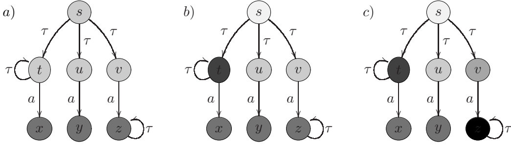
Figure 2: Difference between a) \rightleftharpoons_b , b) \rightleftharpoons_b^\lambda , and c) \rightleftharpoons_b^\Delta .
