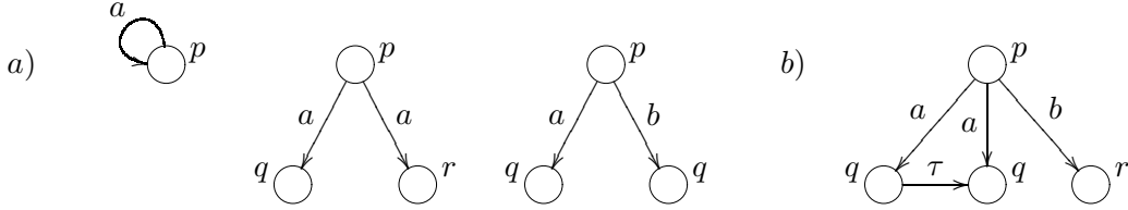
Figure 3: a) Three inconsistent L^2TS s and b) a consistent L^2TS .
