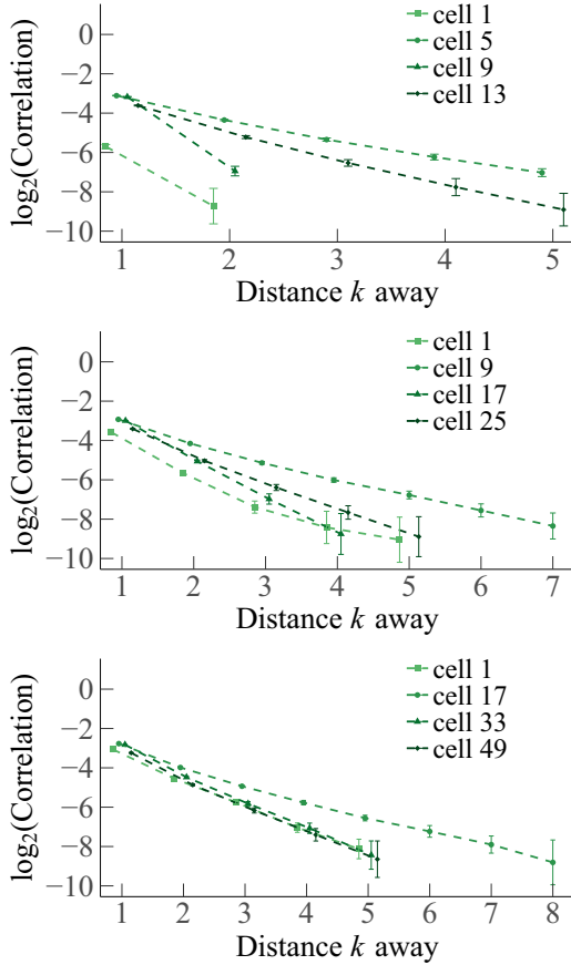
FIG. 5. Decay of correlations, on a log-scale, for the heterogeneous case. From top to bottom we have L = 32, 64, and 128 . For clarity of the figure, the graphs have been shifted horizontally by a small value.
