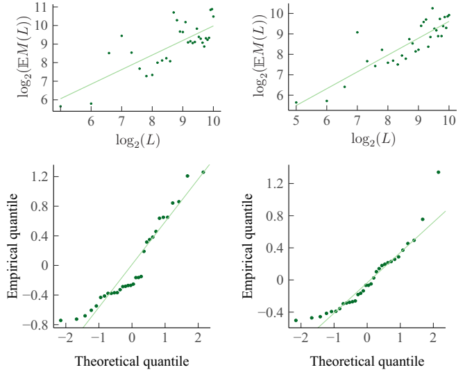
FIG. 11. Illustration results of linear regression. The upper figures show the regression and the lower figures show the corresponding QQ-plots, with the homogeneous case (left) and the heterogeneous case (right).
