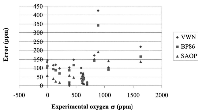
FIG. 3. Residual errors (ppm) in calculated ^{17}\text{O} SAOP NMR chemical shifts, in comparison to VWN and BP86.
