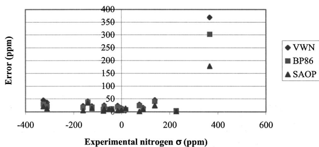
FIG. 2. Residual errors (ppm) in calculated ^{14}\text{N} , ^{15}\text{N} SAOP NMR chemical shifts, in comparison to VWN and BP86.
