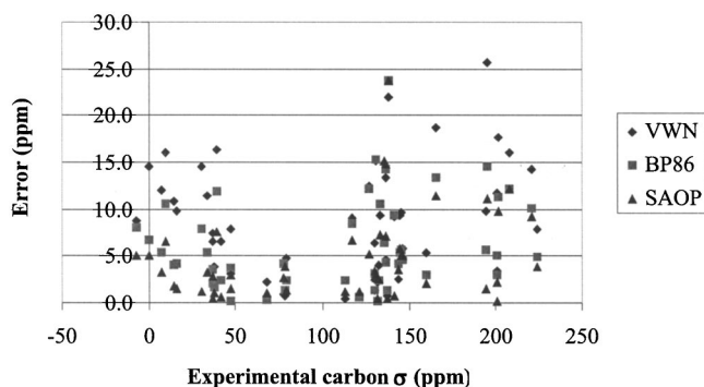
FIG. 1. Residual errors (ppm) in calculated ^{13}\text{C} SAOP NMR chemical shifts, in comparison to VWN and BP86.
