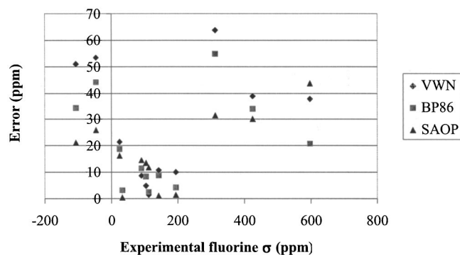
FIG. 4. Residual errors (ppm) in calculated ^{19}\text{F} SAOP NMR chemical shifts, in comparison to VWN and BP86.
