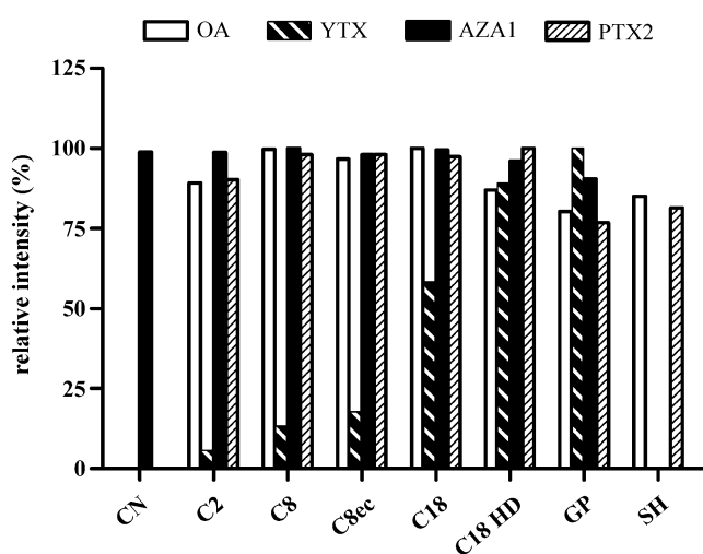
Fig. 4 Sorbent screening using the Symbiosis Pharma automated SPE system. Highest signal intensity per individual toxin set at 100%. Wash with 20% v v^{-1} methanol/water elution with 1% v v^{-1} NH 4 OH in methanol
