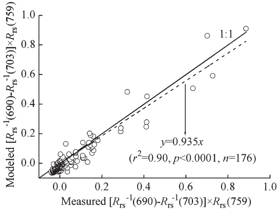
Fig. 8. Comparison of measured and modeled [R_{\text{rs}}^{-1}(690) - R_{\text{rs}}^{-1}(703)] \times R_{\text{rs}}(759) .
