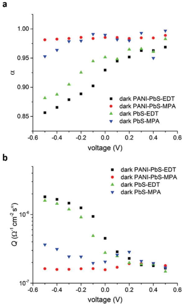
Fig. 4: (a) \alpha values and (b) Q values plotted against bias voltage for PbS-EDT devices with PANI : PSS interlayer (black squares) and without (green triangles), as well as for PbS-MPA with (red dots) and without PANI : PSS interlayer (blue triangles). \alpha and Q were obtained from fits using the circuit model displayed in Figure 2.
