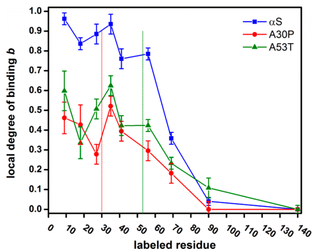
Figure 4. Comparison of the local binding affinity b of \alpha S (blue), A30P (red) and A53T (green) at different labeled residues of \alpha S in the presence of LUVs mimicking the IMM. Full set of fit parameters is shown in Table S5.
