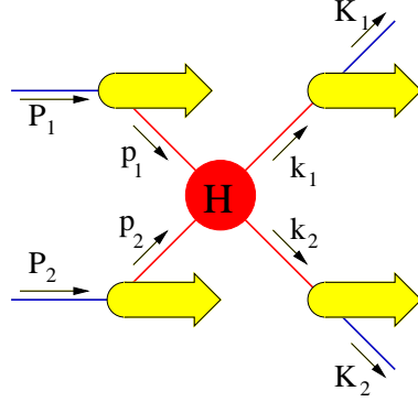
Figure 2. Schematic illustration of the contribution of a hard subprocess, parton ( p_1 ) + parton ( p_2 ) \rightarrow parton ( k_1 ) + parton ( k_2 ), to the (2-particle inclusive) scattering process hadron ( P_1 ) + hadron ( P_2 ) \rightarrow hadron ( K_1 ) + hadron ( K_2 ) + X, at the level of the amplitude. The process being hard implies for the hadronic momenta P_1 \cdot P_2 \sim P_1 \cdot K_1 \sim Q^2 , etc.
