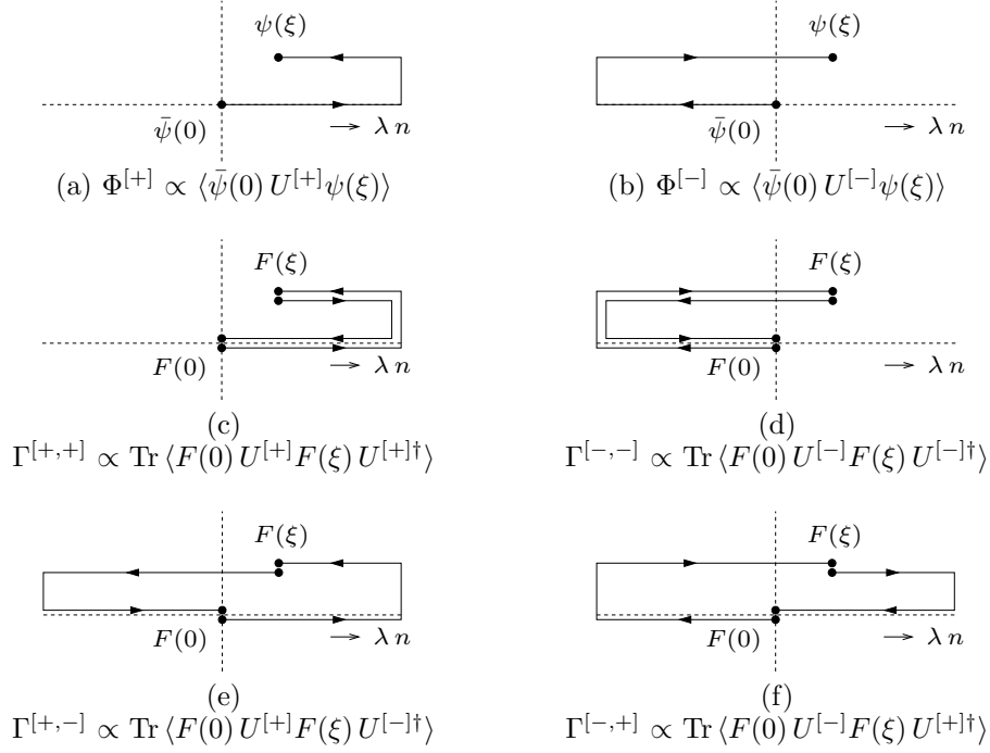
Figure 1. Simplest structures (without loops) for gauge links and operators in quark correlators (a)–(b) and gluon correlators (c)–(f).
