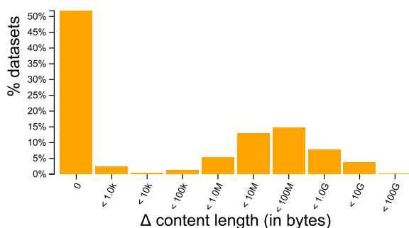
Fig. 10. Invalid HTTP Content Lengths.
