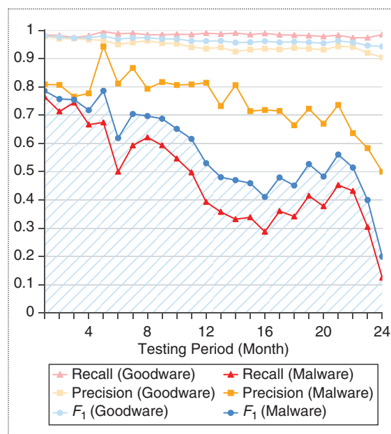
Figure 1. The performance decay in several metrics of a malware detection model trained at month 1 when evaluated against the new malware and benign software of each month for 24 months (adapted from Pendlebury et al. 8 ). Performance numbers are shown both for detecting malware and detecting benign software (goodware, in light colors), respectively. The shaded area under the F_1 curve for malware detection is the area under time, measuring robustness against decay.
