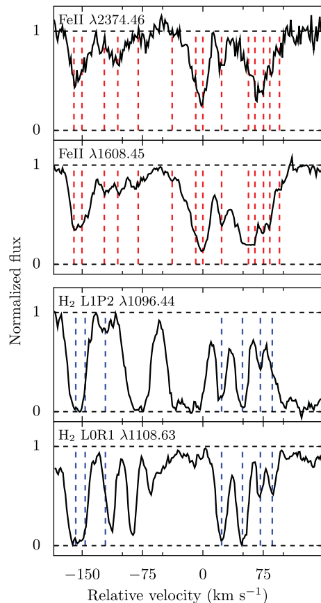
Figure 1. Two H_2 and two Fe\ II transitions are displayed on a common velocity scale, centred at z_0 = 2.426\ 3230 . In the H_2 velocity profile seven distinct features are visible, while the Fe\ II profiles consist of at least 14. Note that the third velocity component from the left in the H_2 LOR1 profile and the rightmost component in the H_2 L1P2 profile are blended with other intervening transitions in Lyman \alpha forest. Due to such blends, the signal of at least seven absorption components is evident only when multiple H_2 transitions are explored simultaneously.
