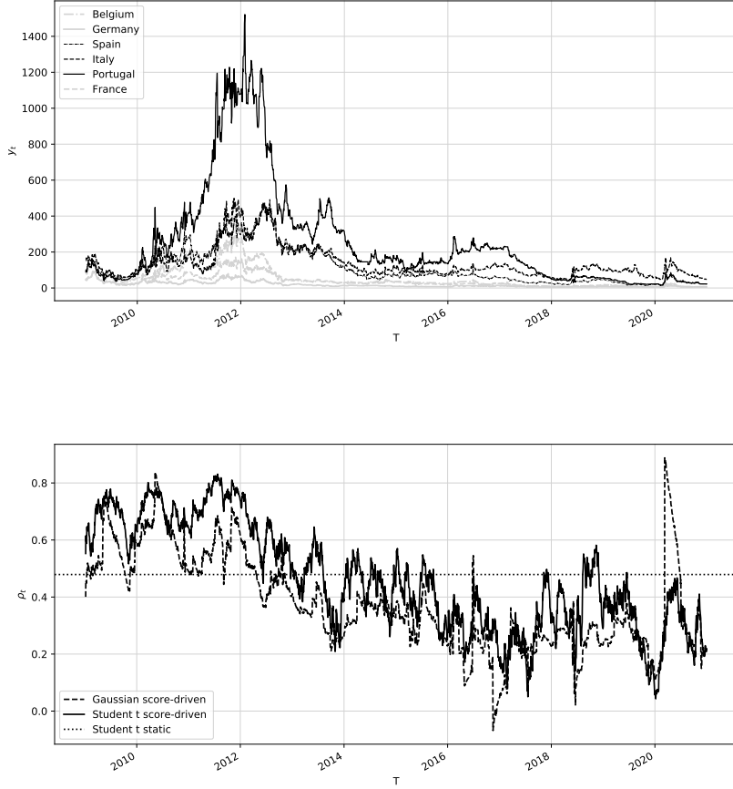
Figure 3: Empirical illustration: score-driven dynamic spatial Durbin model. CDS spreads data for six countries (top) and estimated spatial parameter (bottom).
