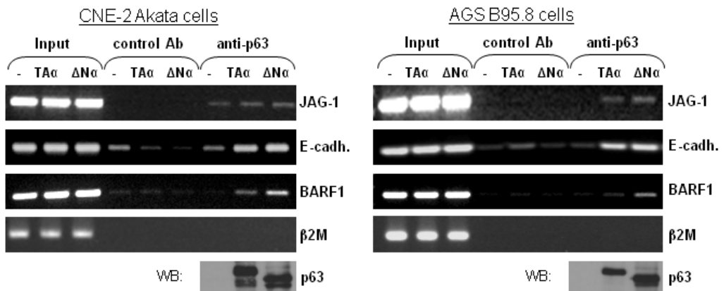
Figure 3. \Delta Np63 \alpha directly complexes with the BARF1 promoter. ChIP assays were performed using extracts from CNE-2 Akata and AGS B95.8 cells transfected with the TAp63 \alpha isoform, the \Delta Np63 \alpha isoform, or a control expression vector (-). p63 was immunoprecipitated by a control antibody or a non-isotype specific anti-p63 antibody, and coimmunoprecipitated DNA was PCR amplified. JAG-1 and E-cadherin served as positive controls for p63 binding and beta-2 microglobulin ( \beta 2M) served as negative control. The band in lane 9, indicates that the promoter region DNA is precipitated with \Delta Np63 \alpha .
