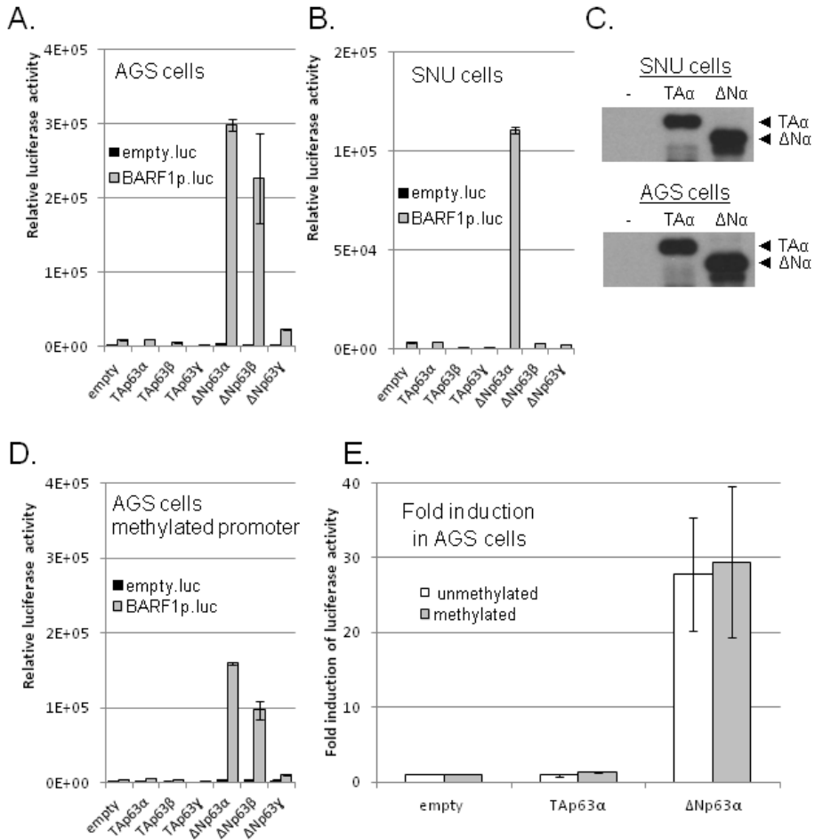
Figure 2. The BARF1 promoter reporter construct is transactivated by the \Delta Np63 \alpha isoform.
