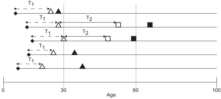
Figure 1. Presentation of the high-grade lesions (CIN2/3) and cervical cancer data. ◆ denotes A_{HPV} , the age of human papillomavirus (HPV) infection based on the age-specific HPV incidence in the Netherlands; \Delta is A_{CIN} , the age of CIN2/3 lesion development (unobserved); \blacktriangle gives the age of CIN2/3 lesion detection (from the nationwide histo- and cytopathology registry); \square is A_{CA} , the age of cervical cancer development (unobserved) and \blacksquare denotes the age of cervical cancer detection (Dutch cancer registry). Between the dotted lines, women are every five years invited to participate in the national screening program. A woman progresses from A_{HPV} to A_{CIN} in T_1 years, and from A_{CIN} to A_{CA} in T_2 years.
