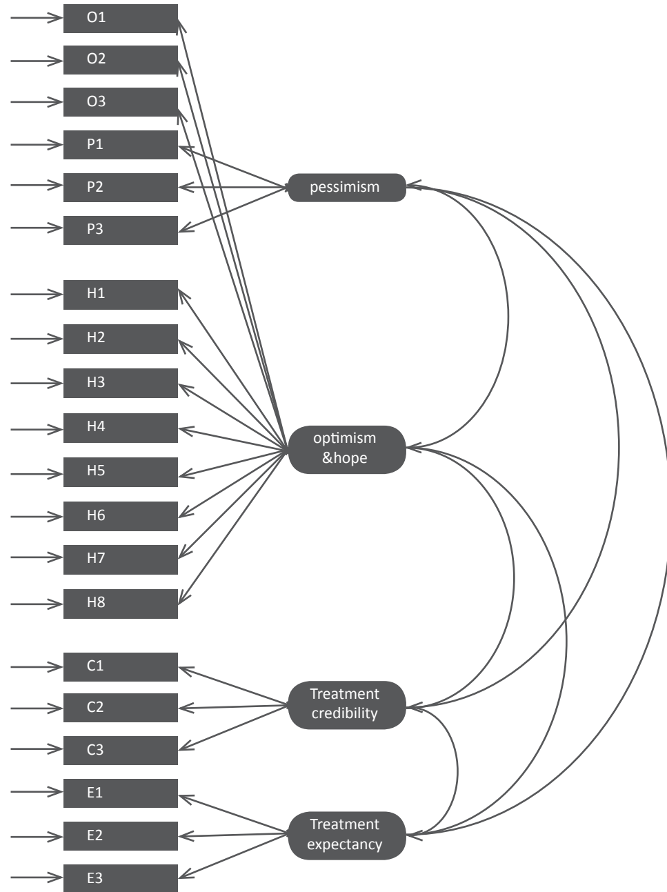
Additional figure 2: Post-hoc model 2, four factor model in which the optimism and hope items load on one factor
