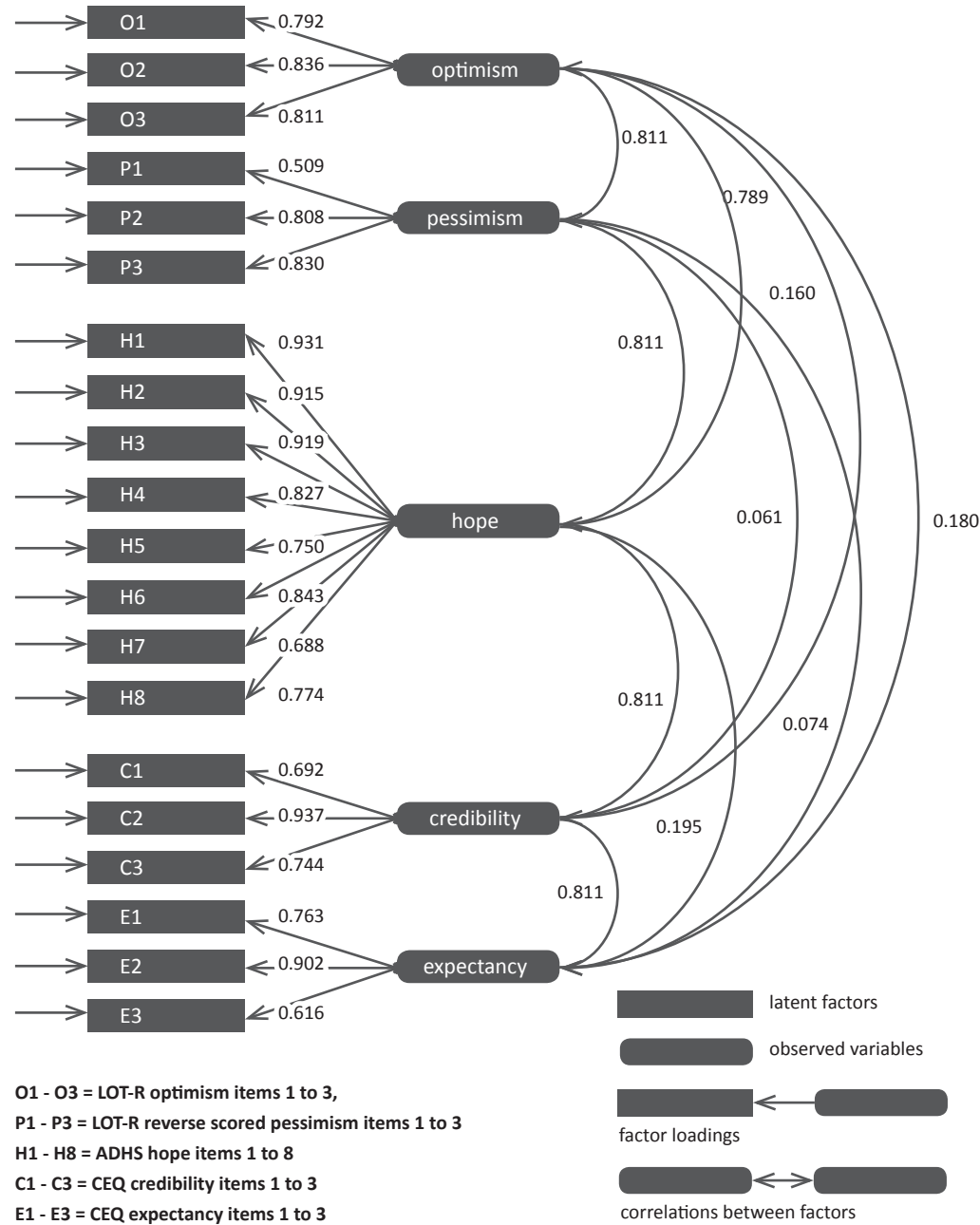
Figure 1. Path diagram and standardized factor loadings and correlations between factors for the 5 factor model
