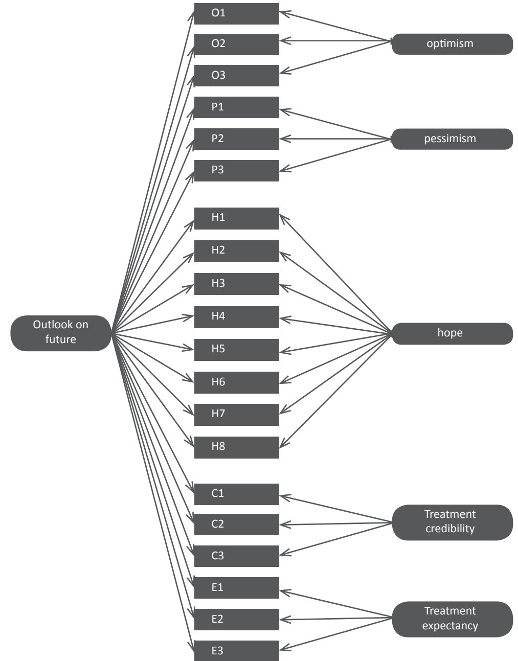
Additional figure 3: Post-hoc model 3, the bifactor model.
