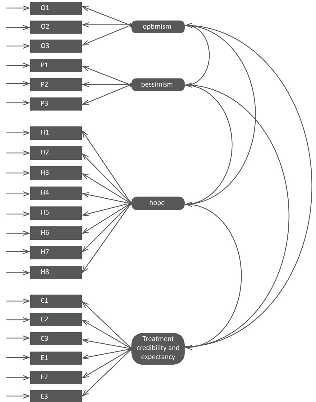
additional figure 1: Post-hoc model 1, four factor model in which treatment expectancy and treatment credibility load on one factor
