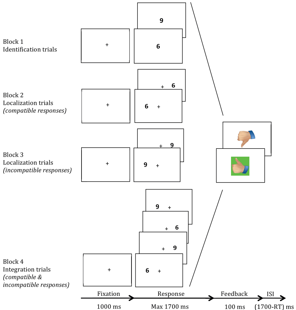
Figure 1. Visual Integration Test procedure
