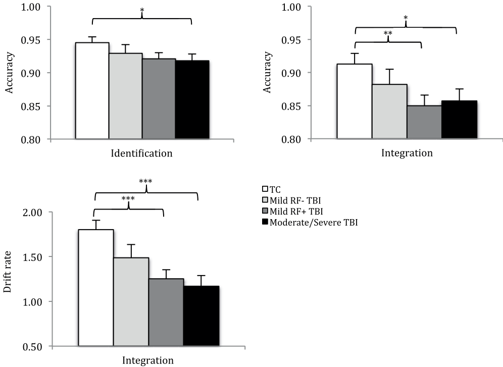
Figure 2. Analyses differentiating TBI severity on visual identification accuracy, visual integration accuracy and visual integration drift rate
