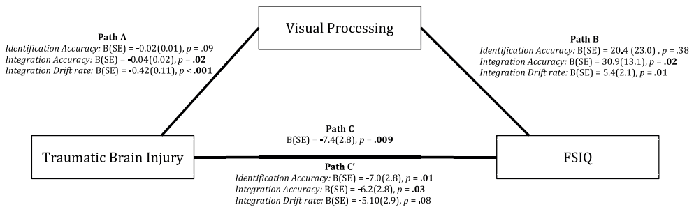
Figure 3. Mediation analysis investigating the roles of visual identification and visual integration in the relation between intelligence impairment and TBI
