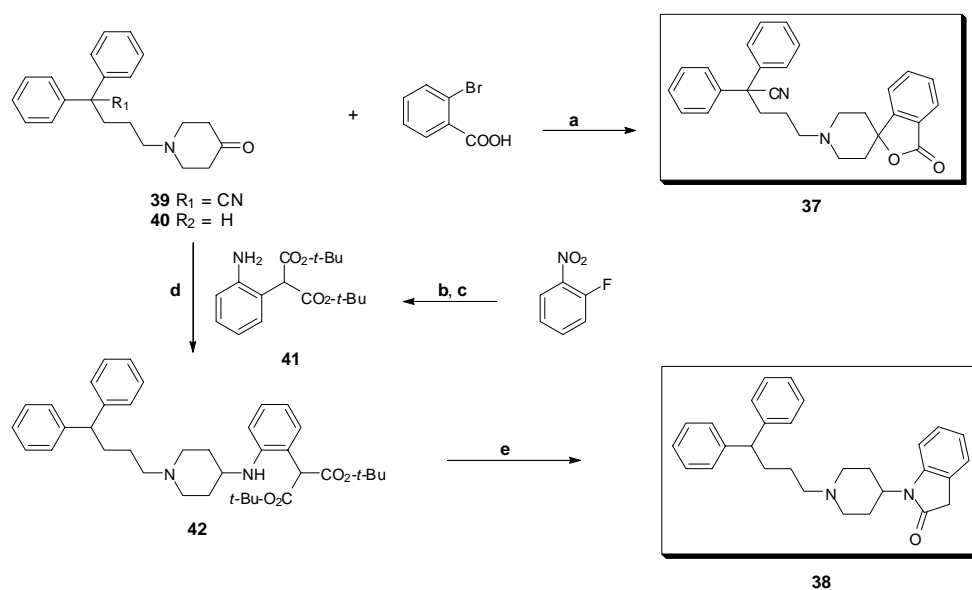
Scheme 3. Synthetic pathway for the synthesis of 37-38 . Reagents and conditions: (a) n -BuLi, THF, -78 °C; (b) Di- t -butylmalonate, NaH, DMF, 90 °C; (c) Pd/C, H 2 , EtOAc; (d) AcOH, NaBH(OAc) 3 , 1,2-dichloroethane; (e) PTSA, toluene, reflux.
