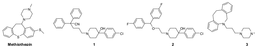
Figure 1. Chemical structure of methiothepin and compound 1-3.
