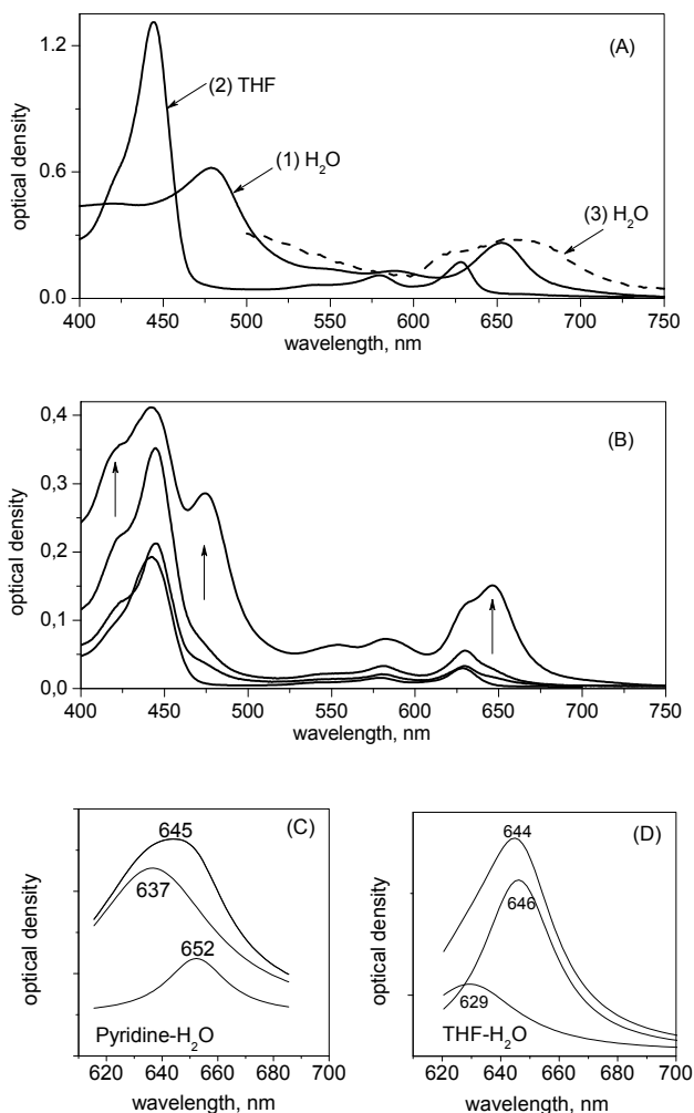
Figure 6.2. Absorption and emission spectra of Pchl. (A) 1 – Pchl absorption in 100% neat water solution recorded in a 1 cm cuvette; 2 – Pchl absorption in THF; 3 – normalized steady-state fluorescence emission with 400 nm excitation. (B) Pchl absorption spectra in THF recorded in 200 \mu\text{m} CaF 2 cell at increasing concentration of pigment. New bands appearing upon concentration increase are indicated by arrows. (C) Lorentzian deconvolution of the Q y absorption band of Pchl in H 2 O containing a few droplets of pyridine and (D) THF.
