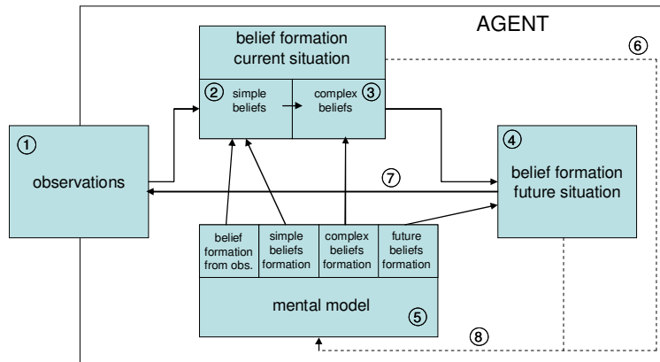
Figure 1. Cognitive model for situation awareness: overview
