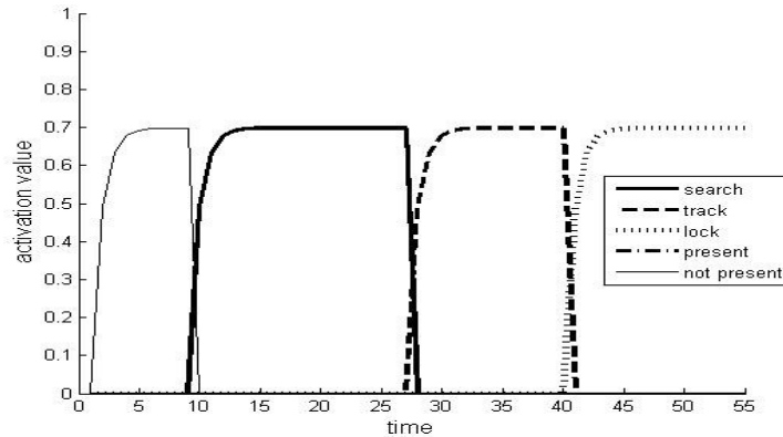
Figure 8. Activation levels of simple beliefs
