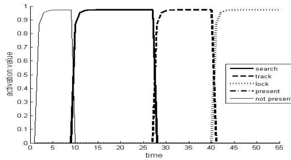
Figure 5. Activation levels of simple beliefs
