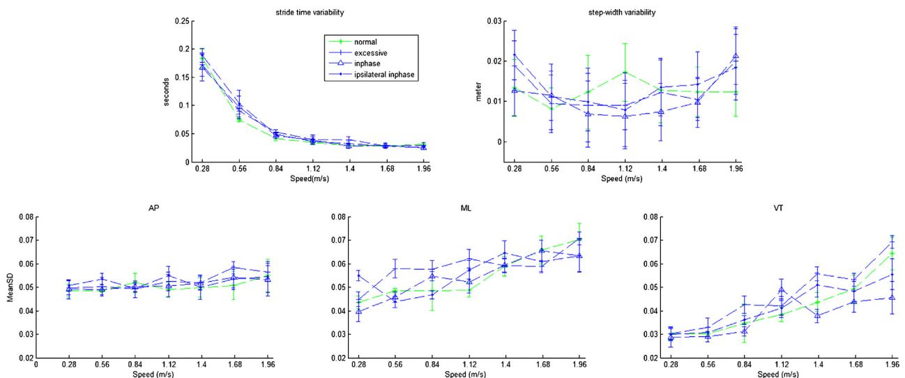
Fig. 3. Group-averaged values of parameters characterizing gait variability. The left upper panel presents stride time variability, the right upper panel step-width variability. MeanSD values are presented at the lower panels from left to right respectively the AP, ML and VT direction. All arm swing instructions are presented, see legend in the left panel. Error bars present standard errors.
