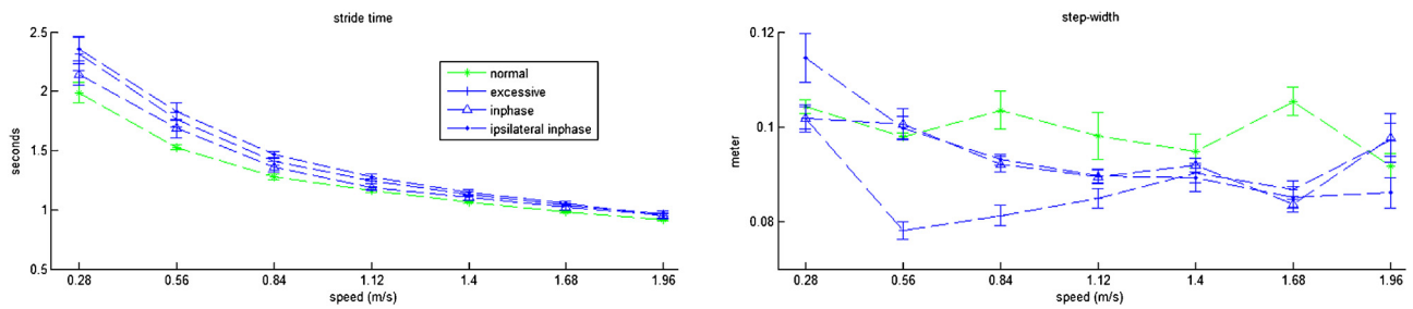
Fig. 1. Group-averaged values of the spatio-temporal measures for all gait speed conditions and arm swing instructions, with stride time in the left panel and step-width in the right panel. Error bars represent standard errors.
