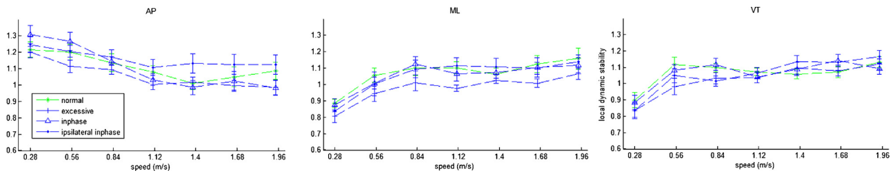
Fig. 2. Dynamic stability quantified as the group-averaged short-term local divergence exponent ( \lambda_s ). The left panel presents \lambda_s for the AP direction, the mid panel for the ML direction and the right panel for the VT direction. Each panel presents all arm swing instructions, see legend in the left panel, and all gait speed conditions. Error bars present the standard error.
