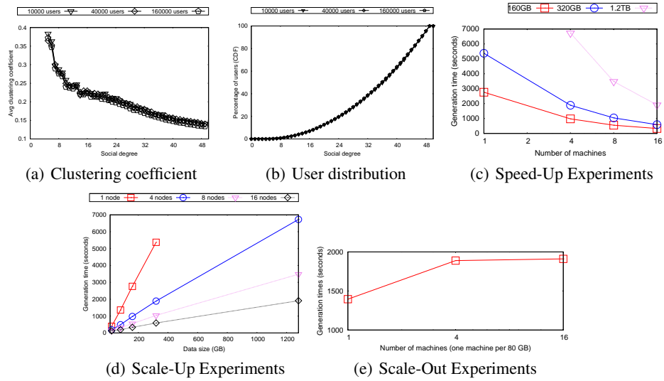
Fig. 5. Experimental Evaluation of S3G2
