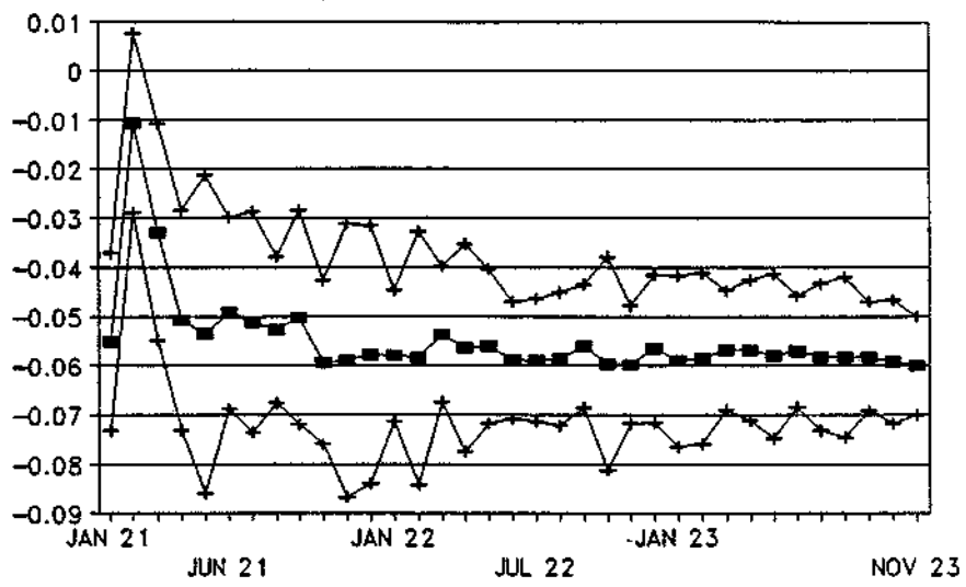
Figure 3 Sequential estimates of beta*
