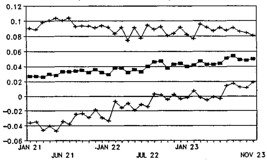
Figure 2 Sequential estimates of gamma2
