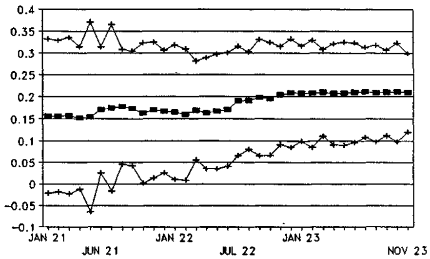
Figure 1 Sequential estimates of gamma1
