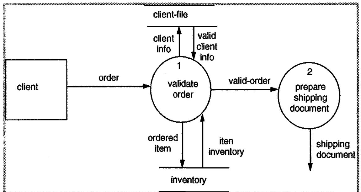
Figure 5. A simple data flow diagram
