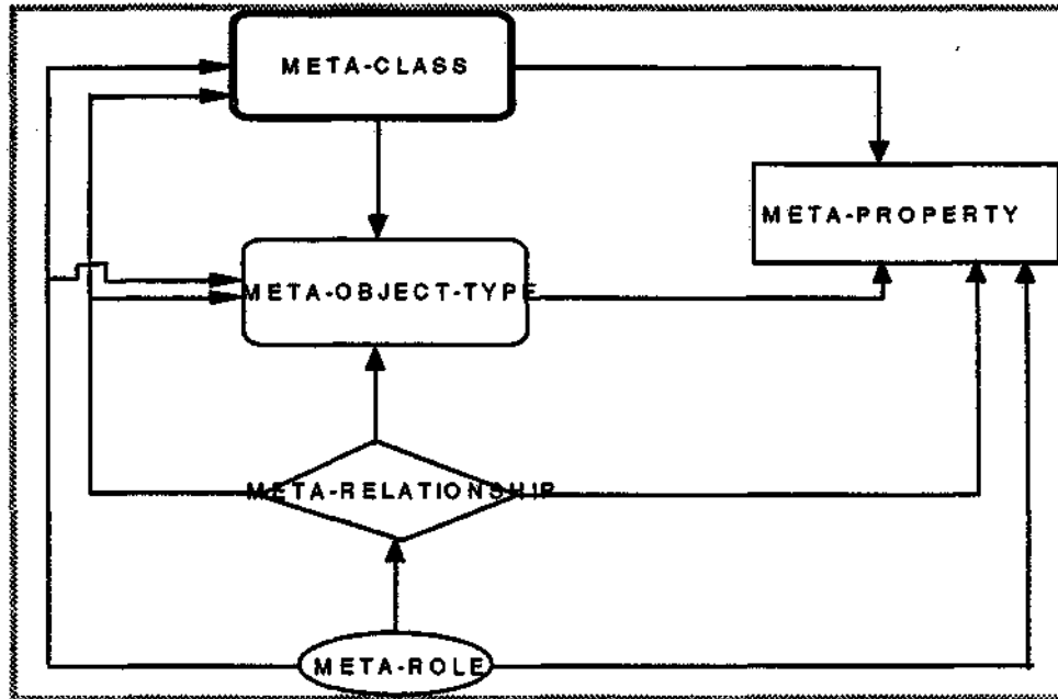
Figure 4. OPRR diagram of a SELC meta-meta model
