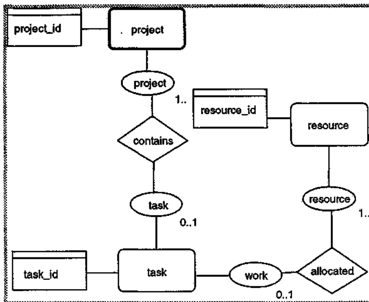
Figure 7. Meta model for project management
