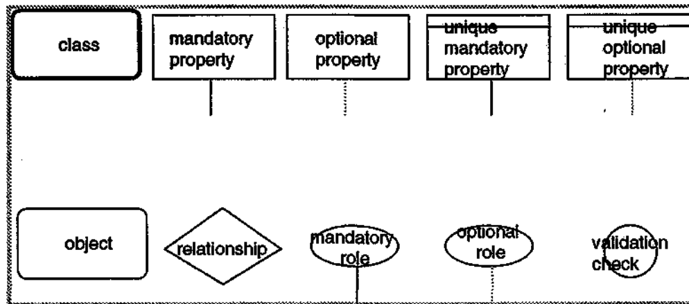
Figure 2. Diagramming notation for OPRR+
