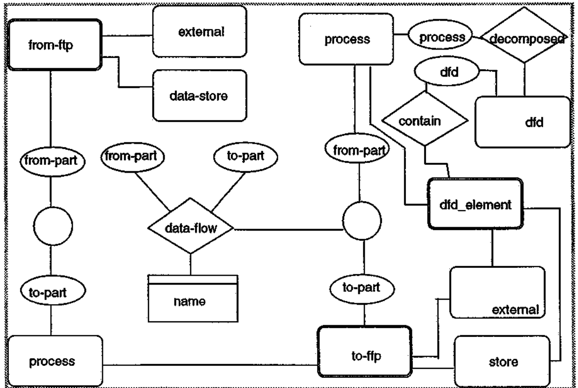
Figure 6. Meta model of data flow diagram
