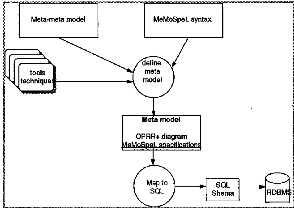
Figure 8. SELC repository implementation
