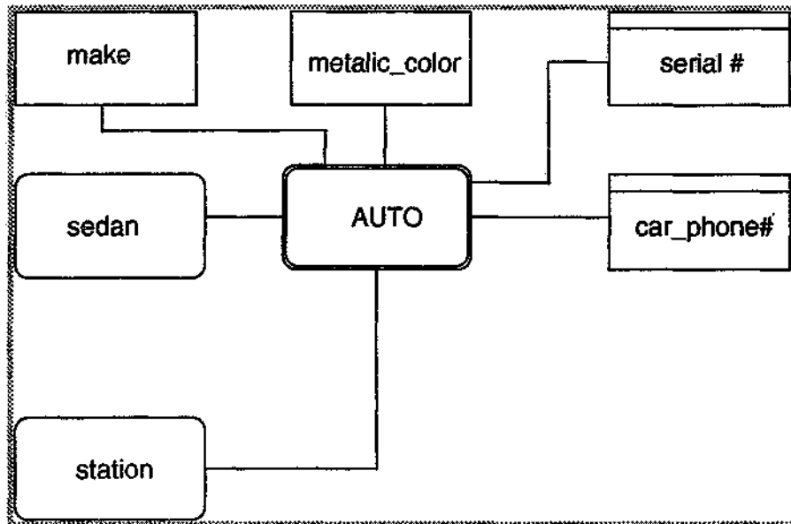
Figure 3. OPRR+ class diagram
