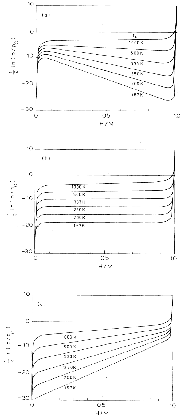
FIG. 2. Pressure-composition isotherms for hydrogen absorption in (a) a perfectly crystallized substance with \Delta=0 , (b) an amorphous substance with \Delta=0.172 eV (2000 K), and (c) an amorphous substance with \Delta=0.345 eV (4000 K). For the three cases E_0 - E_b = -0.086 eV ( -1000 K) and a = -0.345 eV ( -4000 K). In curve (a) the critical temperature is T_c = 1000 K while in (b) T_c = 0 K since 2\Delta = -a . For clarity the plateaus which would result from the application of Maxwell's construction to the isotherms are not shown in Fig. 2(a).
