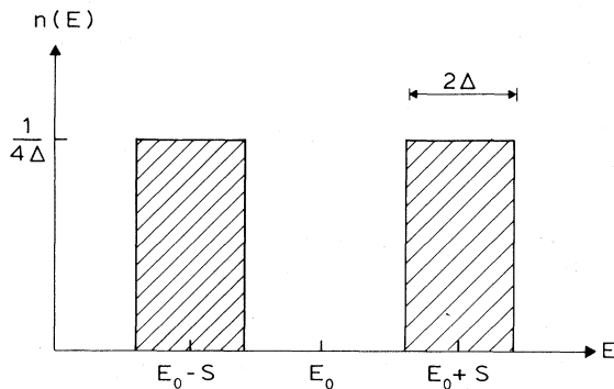
FIG. 4. n(E) for the double-square density-of-sites model.
