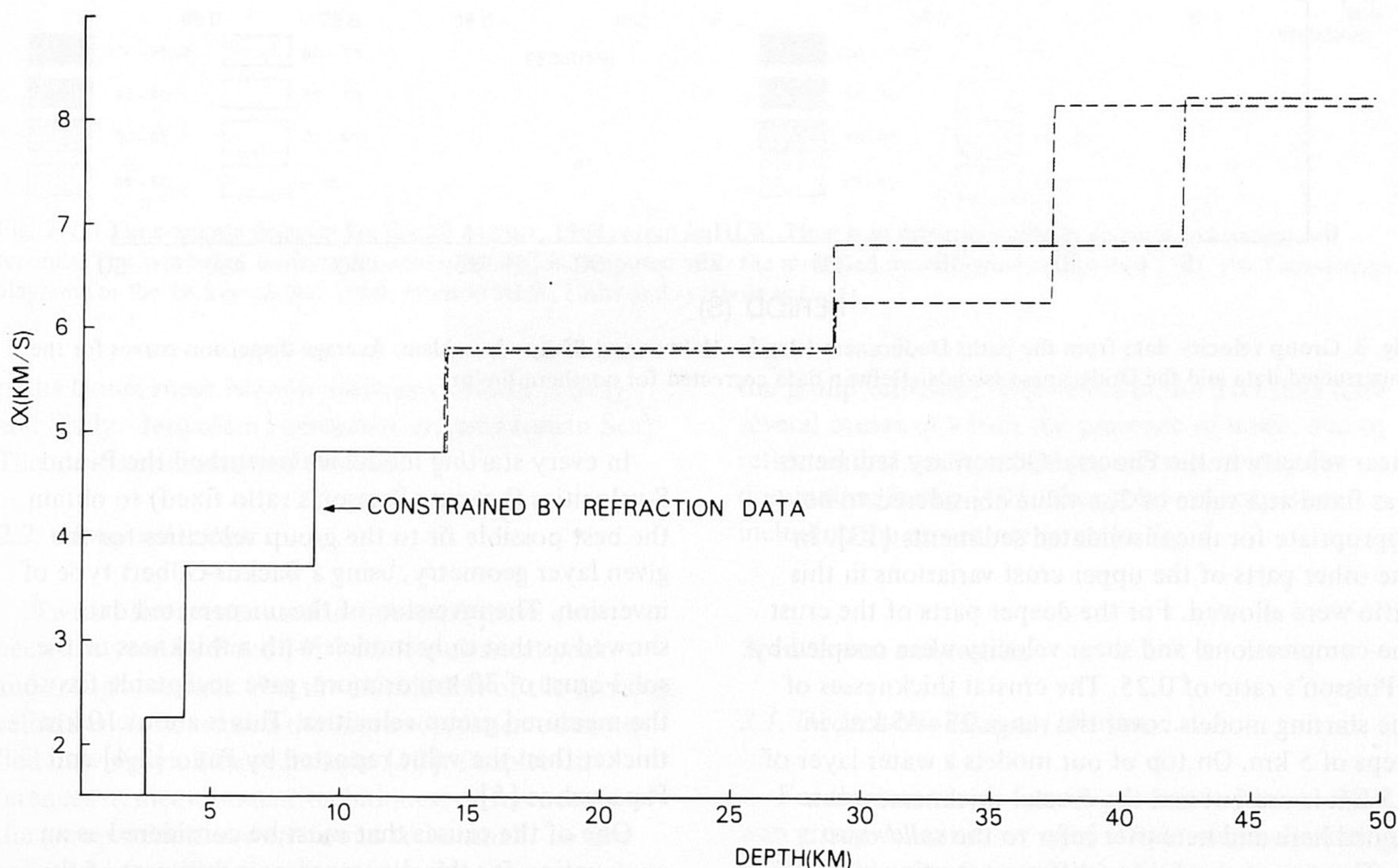
Fig. 4. Inversion results. Shaded area represents the range of velocity-depth distributions allowed by the data, both corrected and uncorrected within their error range. The velocities in the upper part of the crust are constrained by the refraction data. Lines indicate preferred models from corrected group velocities. - - - - -: model with a crustal thickness of 35 km; · - · - ·: model with a crustal thickness of 40 km. For the deeper part of the crust compressional and shear velocities are coupled by a Poisson's ratio of 0.25.
