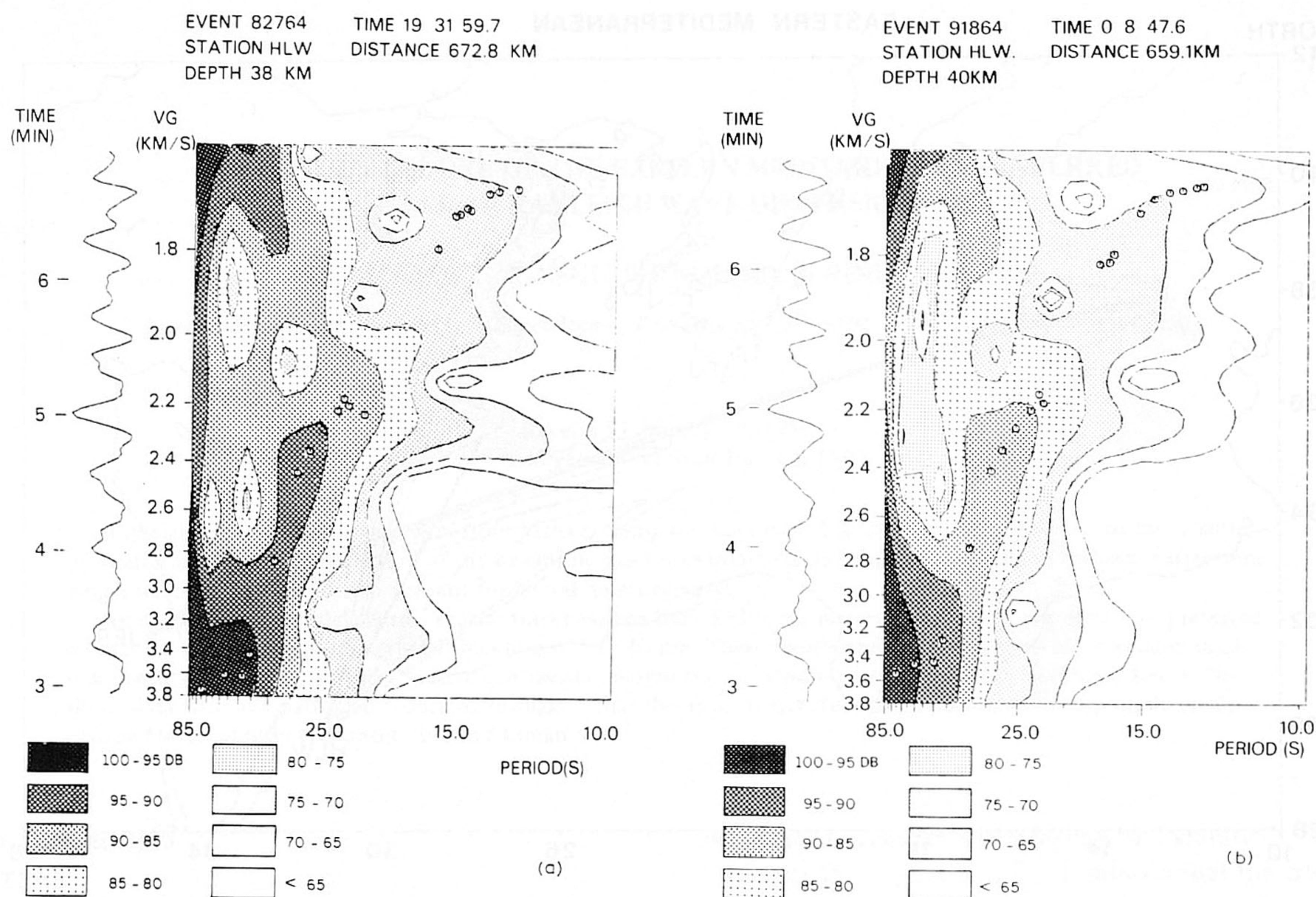
Fig. 2. (a) Time-energy diagram for the 27 August, 1964, event in HLW. Time is in minutes, velocity in km/s and period in seconds. The symbols \odot indicate the group velocities computed with the modified moving-window method [12]. (b) Time-energy diagram for the 18 September, 1964, event in HLW. Units and symbols as in (a).
