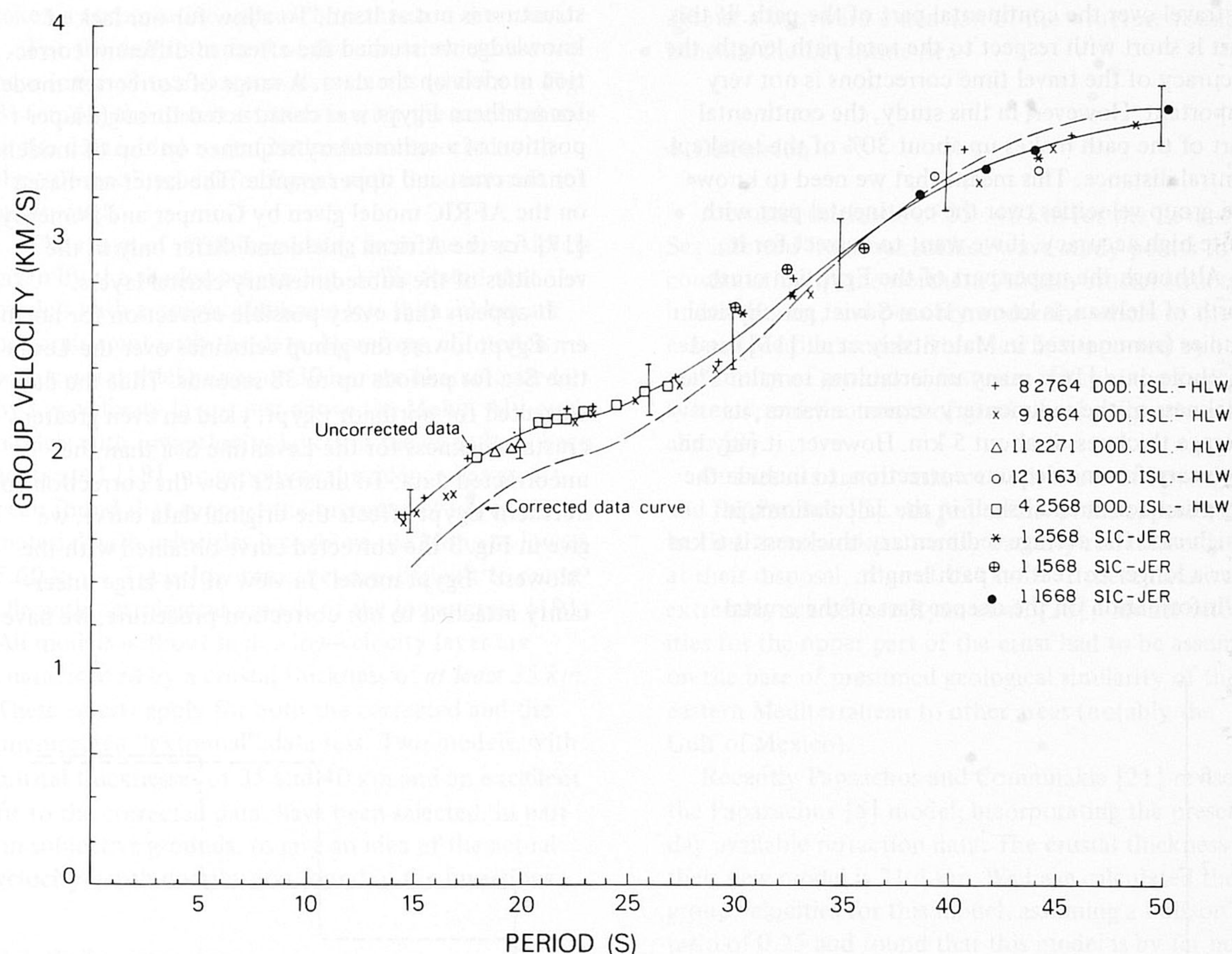
Fig. 3. Group velocity data from the paths Dodecanese Islands–Helwan and Sicily–Jerusalem. Average dispersion curves for the uncorrected data and the Dodecanese Islands–Helwan data corrected for northern Egypt.
