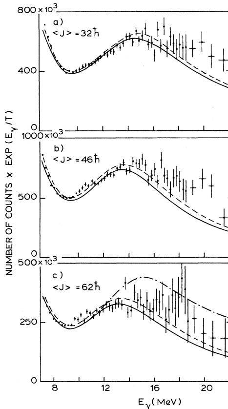
FIG. 2. Prompt high energy \gamma -ray spectra and fits of Figs. 1(a)–1(c) multiplied by the function \exp(E_\gamma/T_{\text{eff}}) with T_{\text{eff}} = 1.95, 1.90, and 1.80 MeV, respectively. The extra dashed-dotted curve is obtained from the solid curve of (a) by normalizing it to the data of (c) at 9 MeV.
