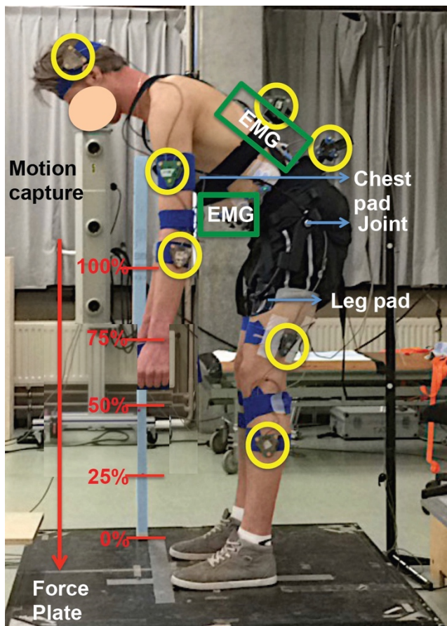
Figure 3. Overview of the experimental setup showing the force plate, marker clusters (yellow), EMG location (green) and an indication of the five hand heights.
