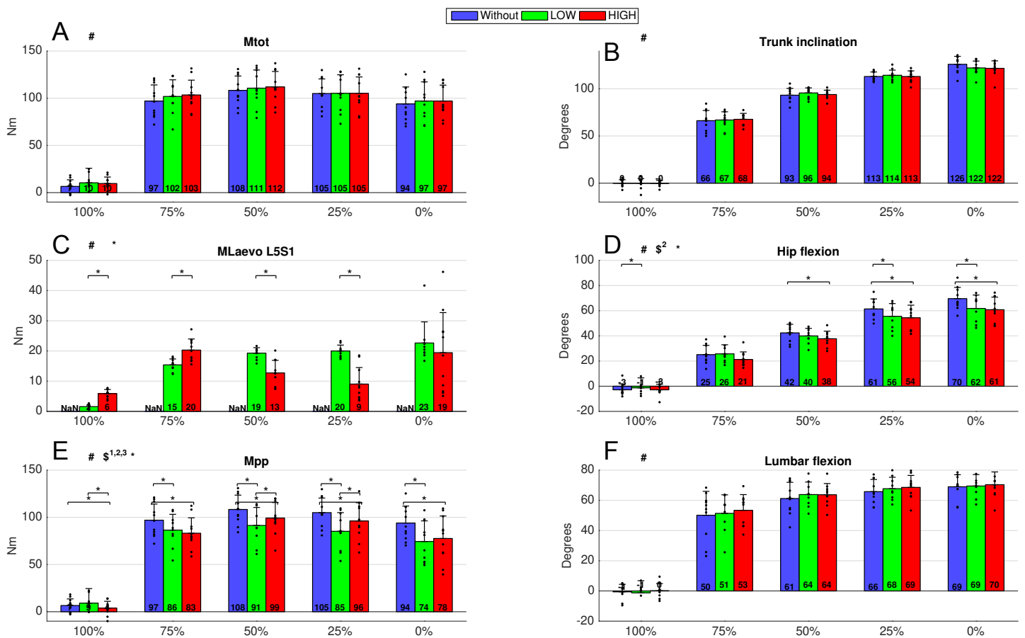
Figure 4. Mean moments ( Mtot , Mlaevo_L5S1 and Mpp in column 1) and angles ( trunk inclination , hip flexion and lumbar flexion in column 2). A main effect of height was indicated with #. A main effect of device was indicated with a $ where 1,2 and 3 stands for significant differences between WITHOUT and LOW, WITHOUT and HIGH and LOW and HIGH, respectively. * indicated a significant interaction between device and height and subsequently, post hoc Bonferroni corrected t-test's were performed. Horizontal bars indicated a significant difference between the two bars.
