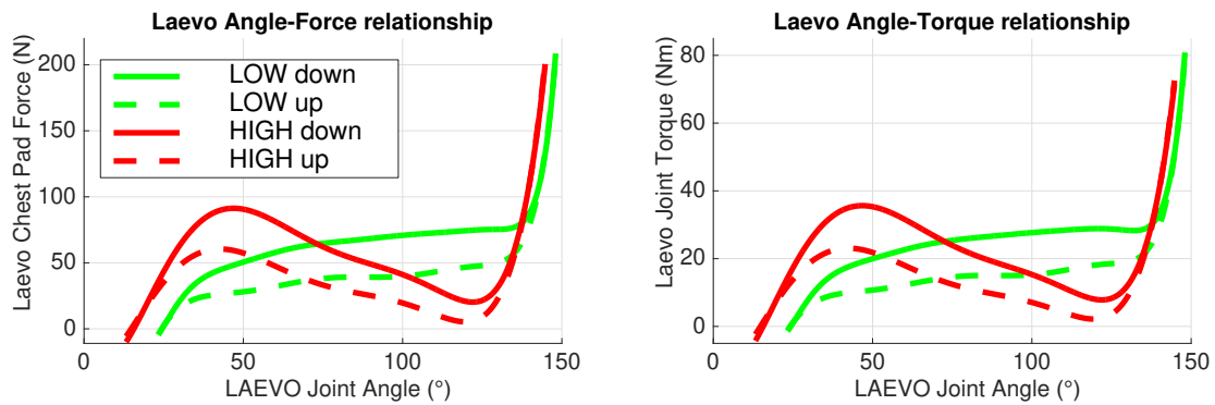
Figure 2. Angle-force relationships measured with two different subjects for both LOW and HIGH. Force was measured using a force transducer placed on the chest pad. Orientation of the chest pad was tracked using a marker cluster. The Laevo joint flexion angle was captured using three LED's (Fig. 1). Note that an offset was present in this flexion angle during upright standing. The Laevo torque was calculated around the Laevo joint using a cross product of the force and the vector from the point of application of the force to the center of rotation of the joint. A substantial difference in support was found between bending (solid) and extending (dashed), due to friction within the system. Beyond the end stop of the Laevo joint, support rapidly increased due to bending of the flexible beams. Note that, during the static bending tasks the Laevo torque was calculated around L5S1 and not around the Laevo joint itself, like in this figure.
