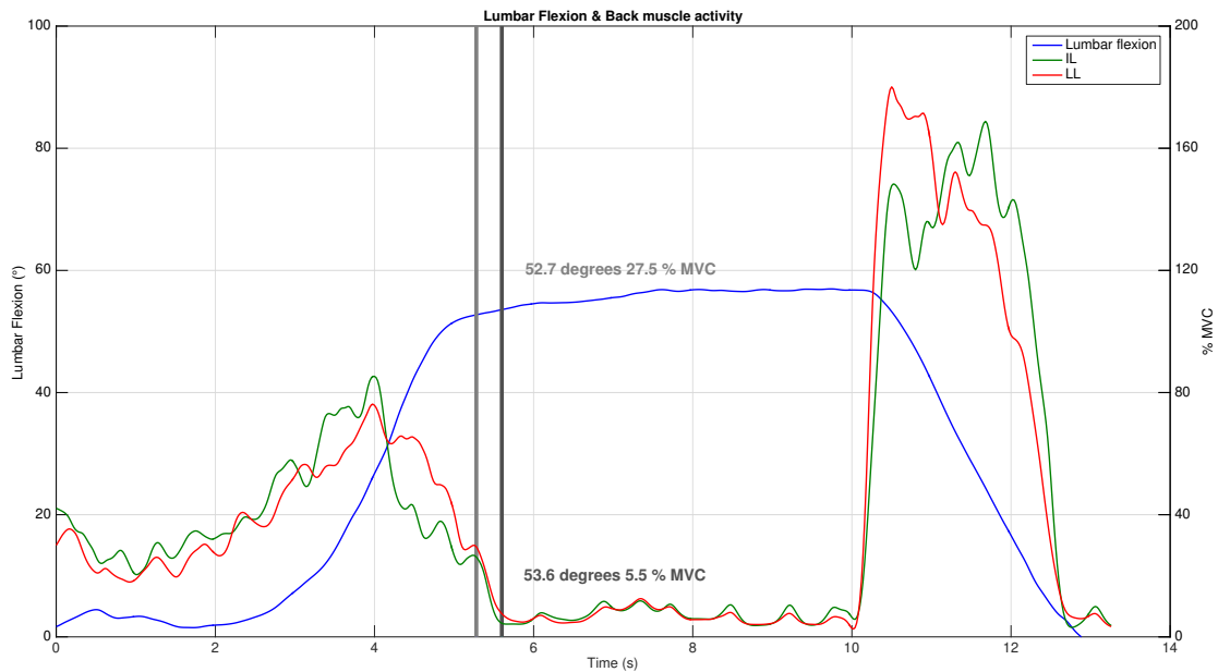
Figure 6. Typical example of a ROM trial showing the relation between lumbar flexion and muscle activity of the two back muscles. Vertical lines show the EMG values at two different lumbar flexion angles.
