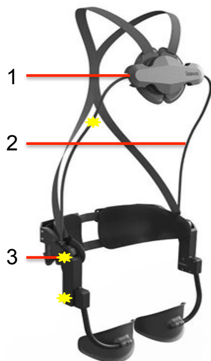
Figure 1. Laevo (V2.4) (Laevo, Delft, The Netherlands). 1) Rotational chest pad, 2) Flexible beam, 3) Spring loaded joint. During the experiments, three LED's were used to measure the Laevo joint flexion angle. The user's trochanter major is to be aligned
