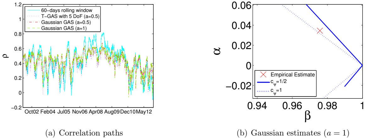
Figure 4: Empirical estimation
